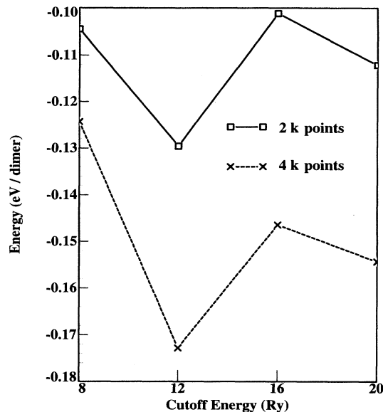
FIG. 15. Convergence of E_{p(2 \times 2)} - E_{p(2 \times 1)_s} as a function of cutoff, using two and four k points. The crosses joined by dashed lines represent calculations performed with four k points (the same calculations as the crosses in Fig. 9). The squares joined by solid lines represent calculations performed using two k points. The two k -point calculations use the same geometries as the corresponding 4 k -point calculations.
