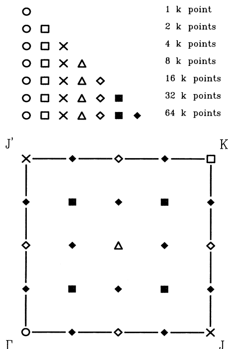
FIG. 3. A quarter part of the p(2 \times 2) Brillouin zone showing the k points used in the various grids. The coarsest grid contains only the point marked with a circle. To double the density, the point marked with an open square is added. Another doubling is achieved by also including the points marked by \times 's, and so on. The numbers of k points refer to the full p(2 \times 2) zone.
