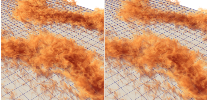
Figure 4: Comparison between volume renderings of temperature with ParaView’s OpenGL GPU RayCastMapper (left), and with NVIDIA IndeX (right).
