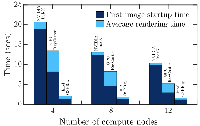
Figure 7: Overview of initial cost and average rendering time per frame.
