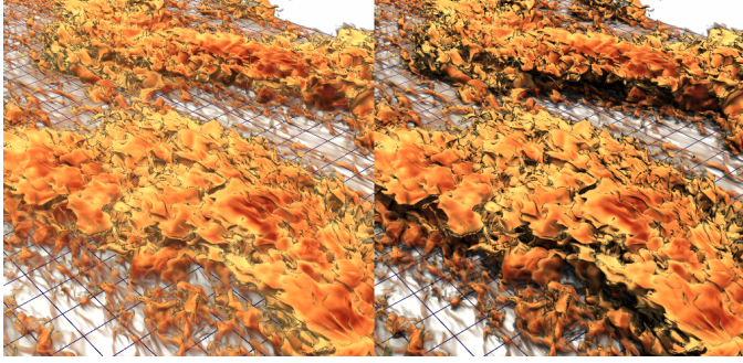
Figure 6: Volume rendering with shading based on gradient estimation (left), and with OSPRay-enabled shadows (right).
