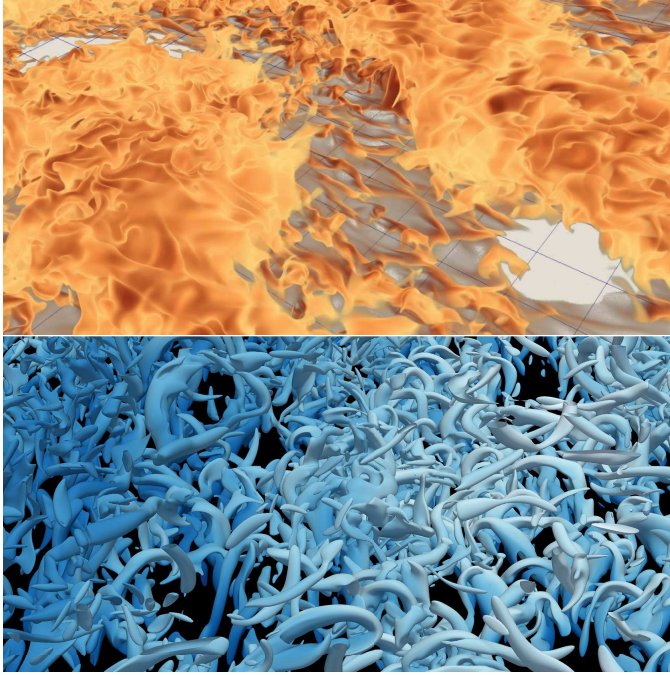
Figure 3: Zoom of an snapshot of the temperature field (top) and the vorticity structures (bottom) at Ra = 2.2 \times 10^6 and Re_w = 6000 .
