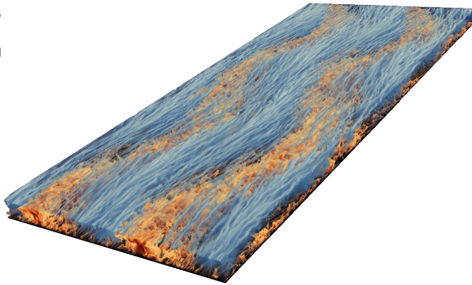
Figure 1: Snapshot of the three-dimensional temperature field of sheared thermal convection at Ra = 4.6 \times 10^6 and Re_w = 6000 [3].
