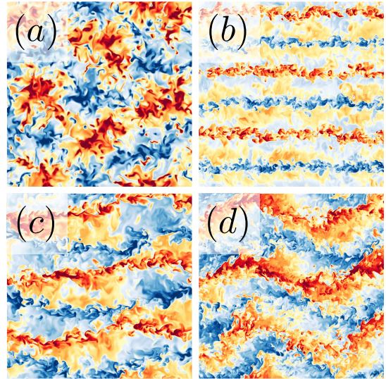
Figure 2: Zoomed snapshots of temperature fields of a sheared and thermally forced flow transitioning through all flow regimes for Ra = 2.2 \times 10^6 and (a) Re_w = 0 , (b) Re_w = 2000 , (c) Re_w = 3000 , (d) Re_w = 6000 , ranging from \theta_{min} (blue) to \theta_{max} (red).
