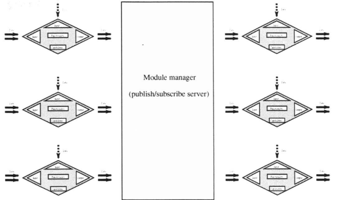
Fig. 6: Data-centric architecture
