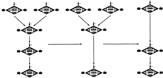
Fig. 7: Architecture transitions
