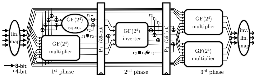
Figure 7.4: The S-box of the raw implementation
