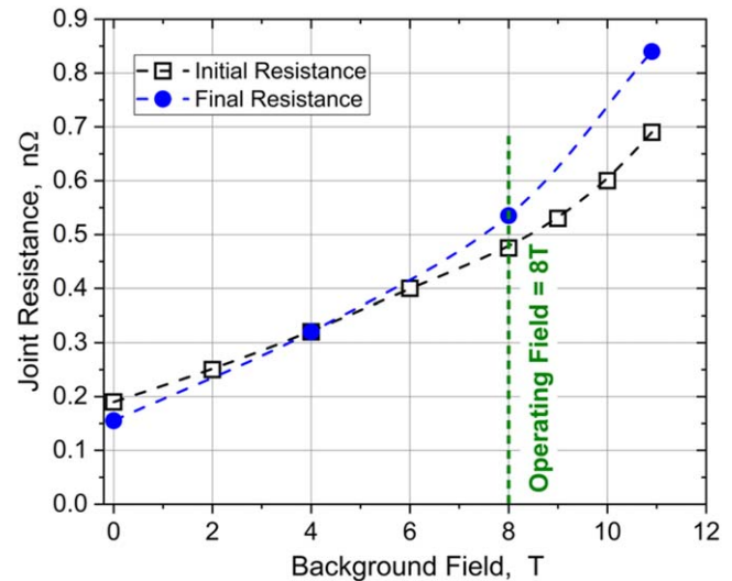
Figure 4. RW2 joint resistance measured at nominal operating current of 63.3 kA in SULTAN test facility. The final resistance was measured after 1000 electromagnetic load cycles and one thermal cycle to room temperature.
