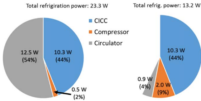
Figure 5. Cryogenic load for one pancake of the TF WP#3 design before and after the optimization. In the reference scenario (left plot), the helium inlet temperature is 4.45 K and pressure head 1 bar, while in the optimized case (right plot) the inlet temperature is 4.0 K and pressure head 0.2 bar.
