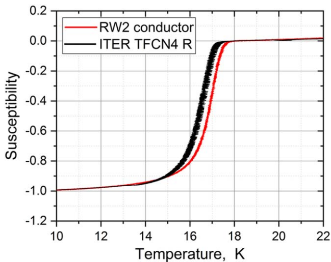
Figure 8. Susceptibility measured in the DEMO TF RW2 prototype conductor and for the ITER TF SULTAN sample.
