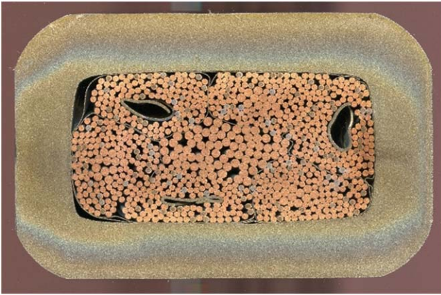
Figure 3. Cross-section of the WR2 low field CICC. The cable is made of 120 Nb 3 Sn wires with 1.0 mm diameter, and of 690/120 Cu wires, with 1.0 mm/1.5 mm diameter, respectively. The steel jacket is 9.5 mm thick. The evident squeezing of the cooling channels requires a design change—either using thicker spirals, or placing them in the interstices between petals.
