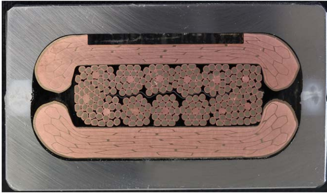
Figure 1. Illustrating photo of the latest RW2 conductor with the full mixed-matrix Cu/CuNi stabilizing profile. The upper rectangular cooling channel was absent in the sample tested in SULTAN (the so-called ‘Full Profile’ sample)—instead, two steel stripes of 0.25 mm thickness were inserted between the steel jacket and the mixed matrix in order to preload the cable in transverse direction (vertical direction in the photo).
