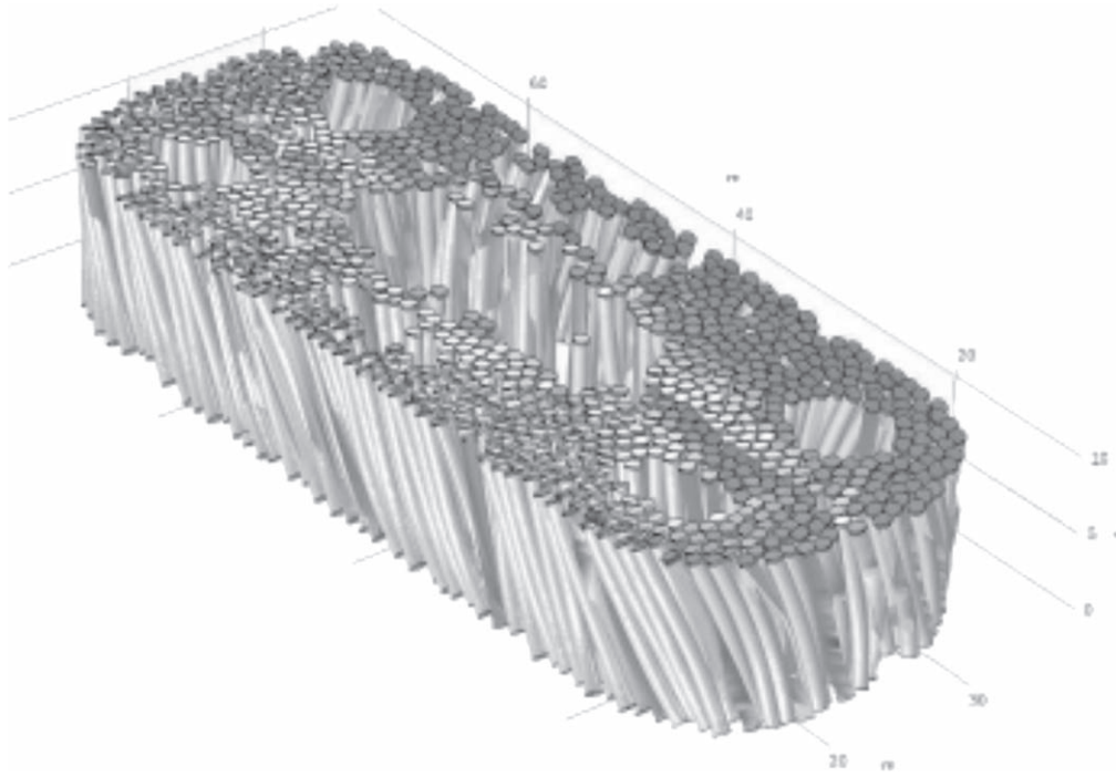
Figure 7. XCT tomographic reconstruction of the Nb 3 Sn strand trajectories. 969 out of 1080 strands were successfully reconstructed.
