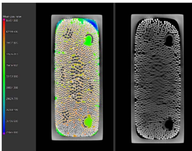
Figure 6. X-ray computer tomography image of the TF WP#2 conductor prototype with slightly reduced jacket thickness. Left plot presents a color-coded void fraction analysis resulting in the void fraction of 0.30 \pm 0.02 in a very good agreement with the nominal specification. Right plot is a typical tomography cross-section—the input for void analysis and strand trajectory reconstruction.
