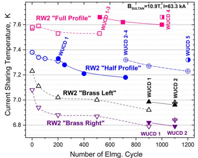
Figure 2. Current sharing temperature measured for four different RW2 conductor samples at 63.3 kA and 10.9 T background SULTAN field. The RW2 ‘Full Profile’ prototype is the latest sample with transverse preload on the cable.
