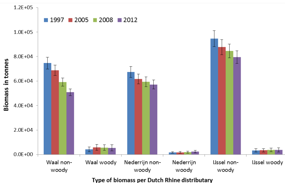
Figure 2. The woody and non-woody biomass production of floodplains along three main river Rhine distributaries in the Netherlands (Waal, Nederrijn and IJssel). Woody indicates the amount of woody biomass (hard wood and soft wood from trees and shrubs) produced; non-woody indicates the amount of non-woody (grass, reed, crops) biomass produced. Error bars indicate standard deviation [4].
