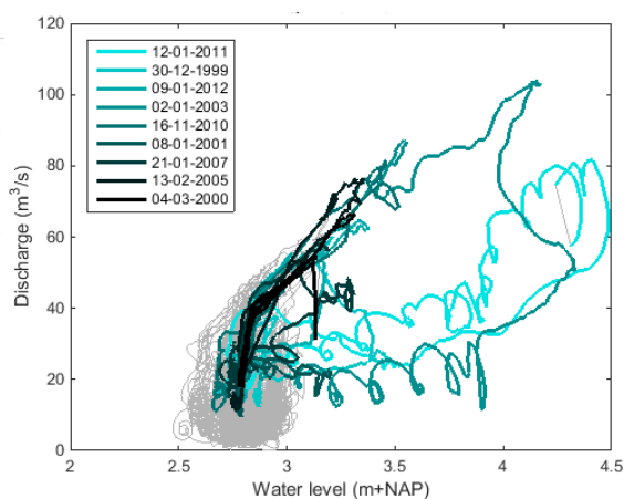
Figure 2. The stage-discharge relation of the Dommel River at the outlet.
