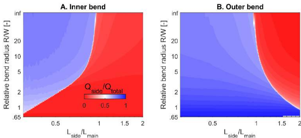
Figure 2. The results of the 1D numerical model for various side channel lengths and bend radii upstream of the bifurcation. (A) The side channel is located in the inner bend, (B) The side channel is located in the outer bend.
