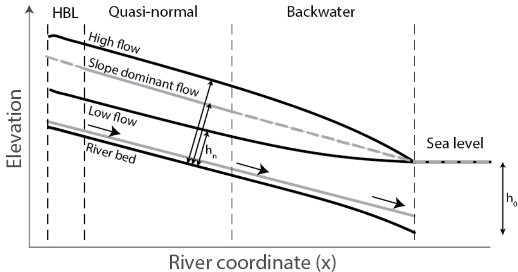
Figure 1. Mean longitudinal river equilibrium profile, divided into three zones. 1) Hydrograph boundary layer (HBL): Transition region in the river where a mismatch in sediment transport rate and transport capacity is corrected for; 2) Quasi-normal flow segment, characterized by a constant slope; 3) Backwater segment, characterized by the presence of backwater curves during high and low flow, resulting into a predominantly convex bed slope.
