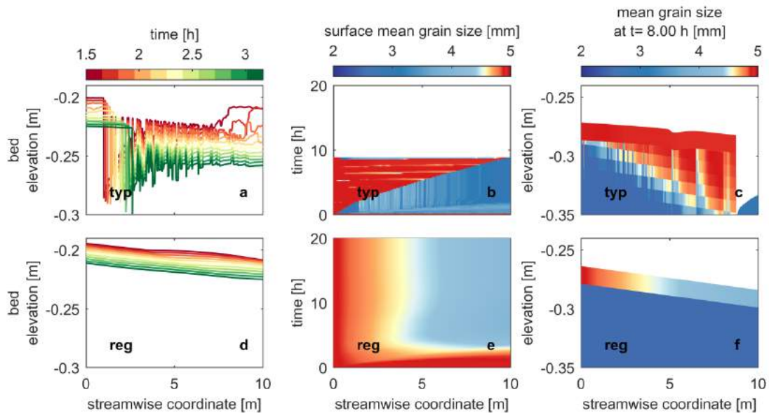
Figure 2. Bed elevation, surface mean grain size, and stratigraphy at the end of two runs. Run I (top) is computed with the typical ('typ') model and Run II (bottom) with our regularization strategy ('reg').
