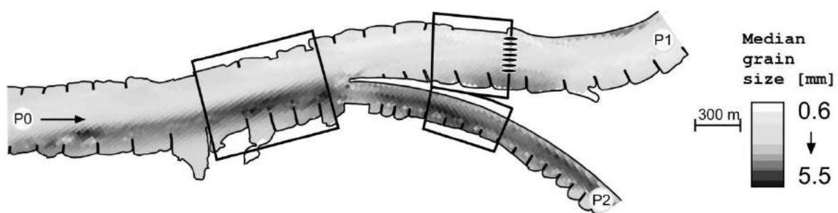
Figure 1. Median bed surface grain size in the Pannerdensch Kanaal, ca. 5 km downstream from the nourishment place (adapted from Frings, 2007).
