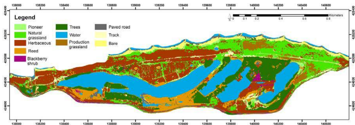
Figure 2. Classification of the Breemwaard based on multi-temporal UAV spectral and height data [3].
