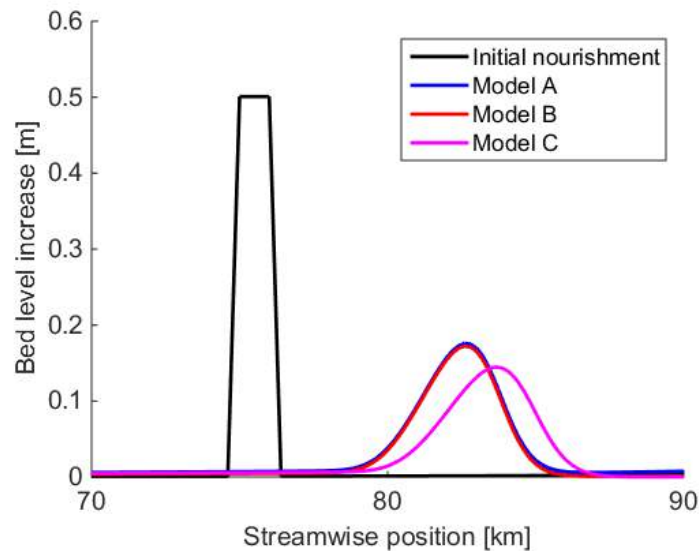
Figure 2. Nourishment displacement after 1 year. Flow model A: Full wave model. Flow model B: Schematized hydrograph with 20 modes. Flow model C: Steady discharge. (Weerdenburg, 2016).
