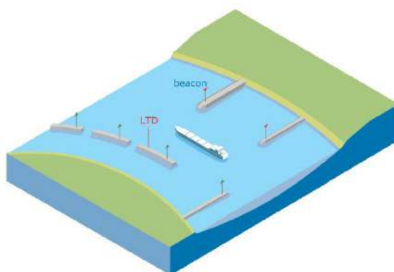
Figure 1. Schematic view of an LTD and the remaining groynes, adapted from (Rijkswaterstaat 2012).
