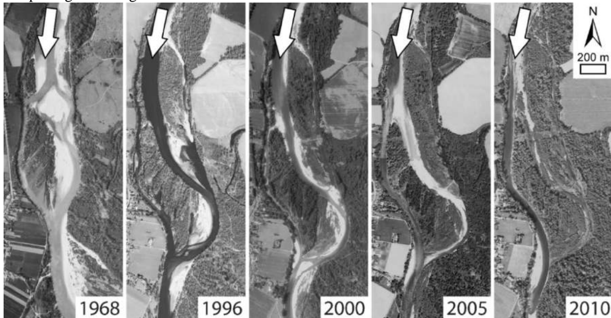
Figure 1. The morphological changes in a two channel system in the River Ain (France) near the village Mollon. (IGN-France, Google Earth)
