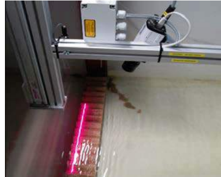
Figure 4. Laser line scanner set-up. A red laser line is projected on the bottom of the flume, which reflection is recorded by a 3D camera (top right).
