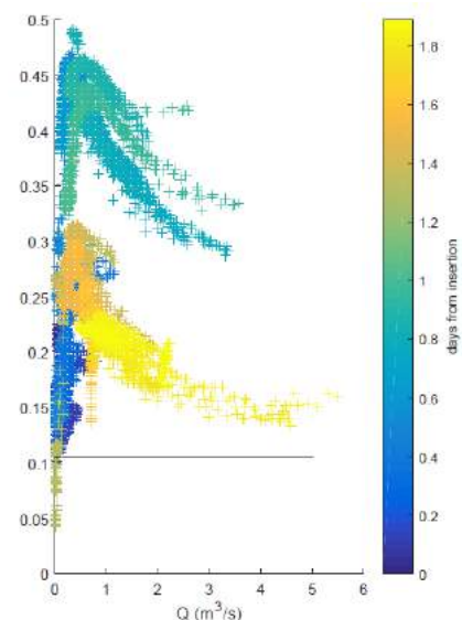
Figure 3. Relation between water level difference and discharge at Leerinkbeek.
