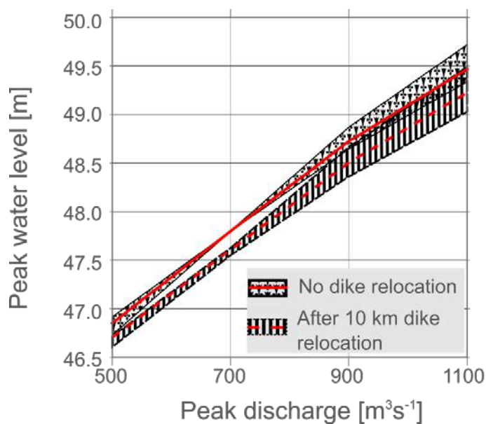
Figure 2. Solid & dashed center lines: ground truth; Envelopes: model results obtained with multiple parameter sets. Both extrapolation and modification (by dike relocation) were found to attribute to increasing uncertainty in prediction. Source: Berends et al. (2016)
