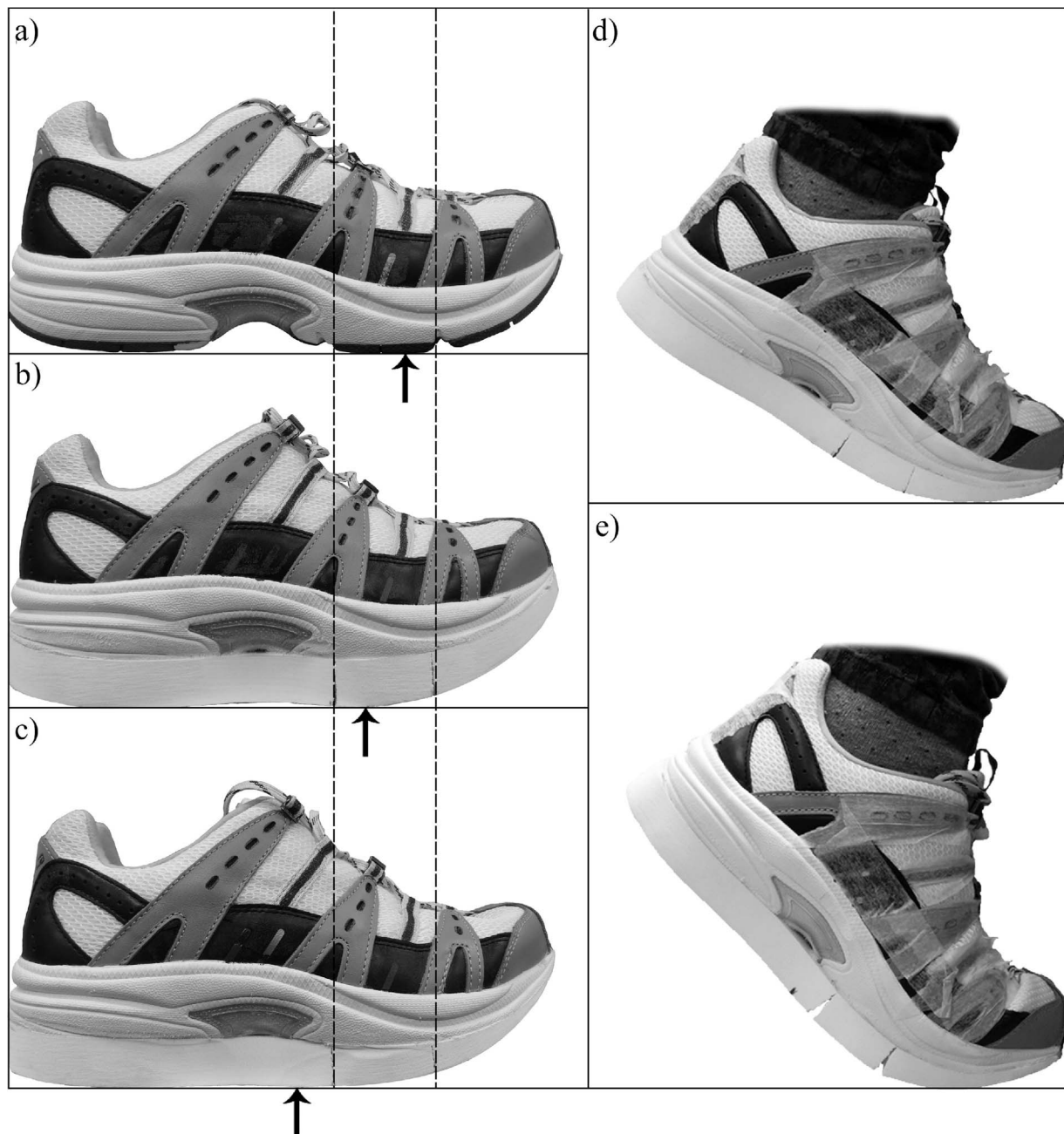
Fig. 1. Shoe modifications. On the left the apex positions for the control (a), modified shoe with apex position at 60% (b) and modified shoe with apex position at 50% (c) are indicated with a black arrow. The dashed lines indicate the position of the notches in the original sole and the cuts in the modified shoes. On the right the difference between the rigid (d) and flexible (e) configurations is shown (both loaded).
