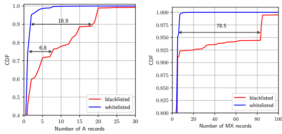
Figure 1: CDF of the number of A records (left) and MX records (right) for snowshoe spam and regular domains
