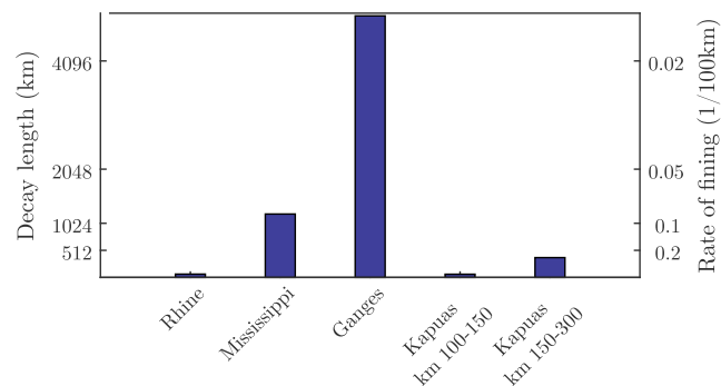
Figure 11. Comparison of downstream fining of bed material between the Kapuas and other large sand bed rivers (adopted from Frings [2008] and original data from ten Brinke [1997], Nordin and Queen [1992], and Singh et al. [2007]).
