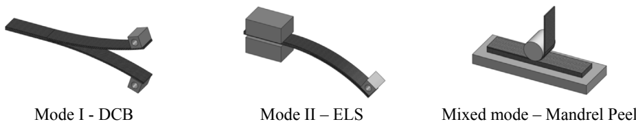
Fig. 1. DCB, ELS, and Mandrel Peel test scheme.
