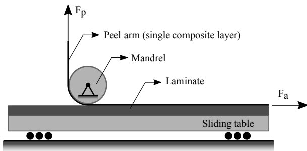
Fig. 6. Schematic view of the mandrel peel test.
