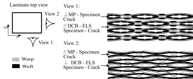
Fig. 5. Schematic view of the stacking sequence and the position and direction of propagation of the crack. For the sake of clarity half of the plies are not shown. MP: Mandrel Peel, DCB: Double Cantilever Beam, ELS: End-Loaded Split.//: Parallel. ⊥: Perpendicular.
