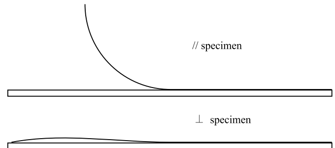
Fig. 7. Schematic view of the mandrel peel specimens showing a typical curvature of the peel arm before testing. //: Parallel. ⊥: Perpendicular.
