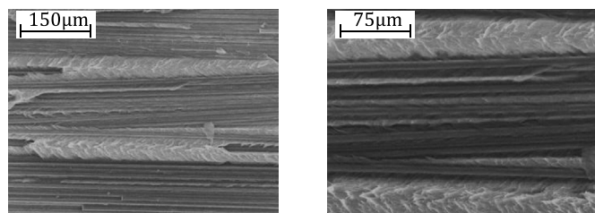
Fig. 19. SEM fractography of a // ELS specimen where the crack propagates from right to left. The right image is a detail and close-up view of the left image.
