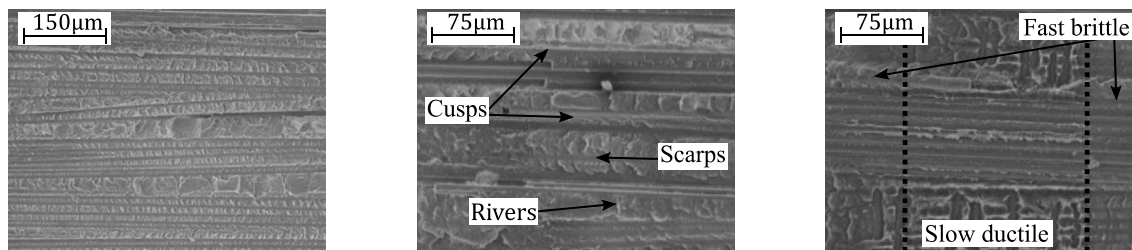
Fig. 18. SEM fractography of a // DCB specimen. The image corresponds to a bundle with the fibres oriented in the same direction of the crack propagation. The crack propagates from right to left. Left) Region of unstable crack propagation. Centre) A zoomed-in look at a region of unstable crack propagation. Right) A zoomed-in look at a stable crack propagation region.
