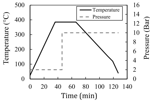
Fig. 4. Schematic representation of the press consolidation cycle.
