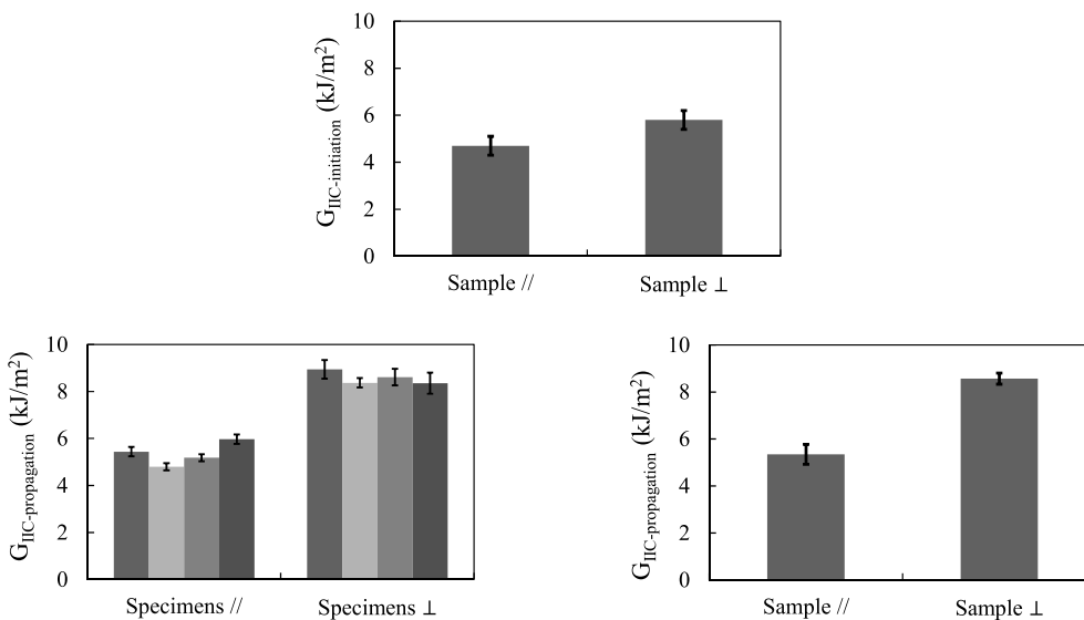
Fig. 11. Upper) Initiation toughness values for the different samples with standard deviation. Bottom-left) Average propagation toughness values for the different specimens with standard deviation. Bottom-right) Average propagation toughness values for the different samples with standard deviation.
