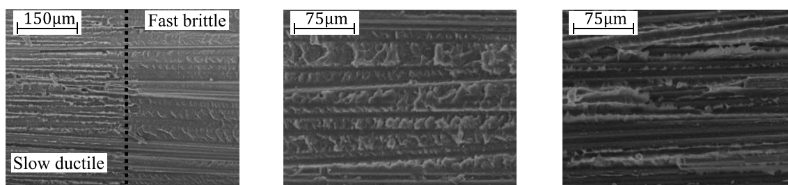
Fig. 20. SEM fractography of a mandrel peel specimen. The crack propagates from right to left. Left) Combination of stable and unstable crack propagation. Centre) Closer look at the region of unstable crack propagation. Right) Closer look at a region of stable crack propagation.
