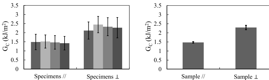
Fig. 14. Left) Average toughness values for the different specimens with standard deviation. Right) Toughness values for the different samples with standard deviation.
