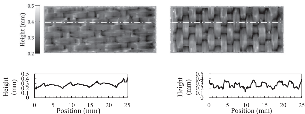
Fig. 17. Fracture surface topology. Left) A DCB parallel specimen. Right) A DCB perpendicular specimen. The white dash-dotted line represents the position where the height was analysed in the lower charts.
