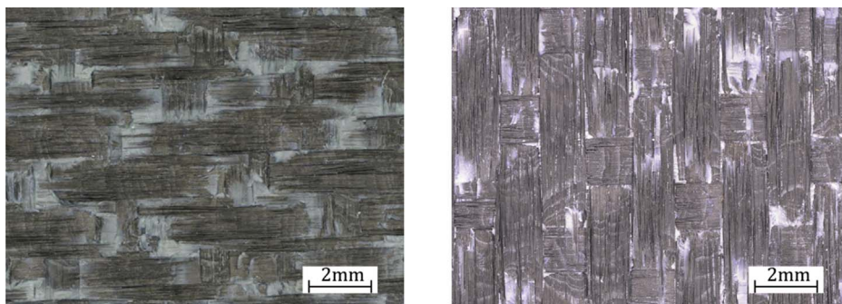
Fig. 15. Fracture surface of two DCB specimens. Left) parallel specimens. Right) a perpendicular specimen. The crack propagation is from right to left.
