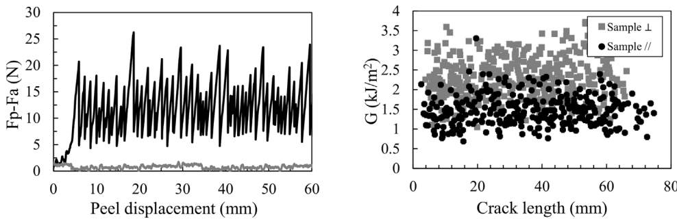
Fig. 12. Left) Force vs. displacement during the mandrel peel test. The black line shows the actual test, while the grey line represents the subsequent run on the (now un-bonded) specimen to determine the friction in the setup. Right) Fracture toughness vs. crack length for all the mandrel peel specimens.
