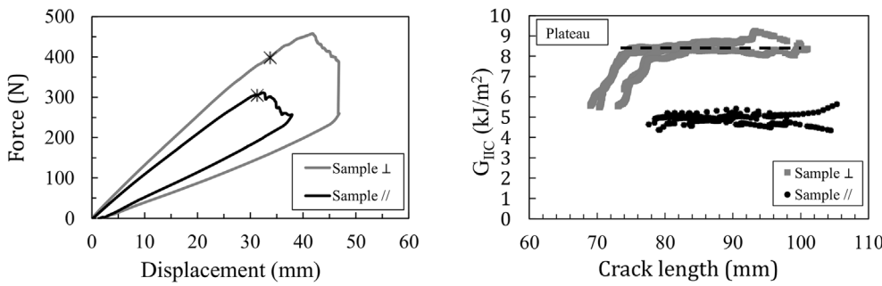
Fig. 10. Left) Force vs. displacement curve. The star symbol represents the position of the crack initiation. Right) Fracture toughness vs. crack length for all the specimens.
