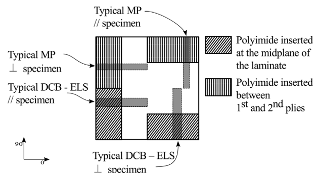
Fig. 3. Schematic view of the position of the polyimide films placed before consolidation. The 0^\circ corresponds to the warp direction. MP: Mandrel Peel, DCB: Double Cantilever Beam, ELS: End-Loaded Split. // : Parallel. \perp : Perpendicular.
