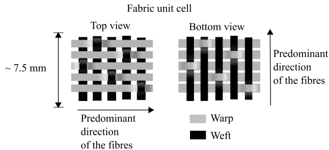
Fig. 2. Schematic view of a unit cell for a 5 harness satin top and bottom view.
