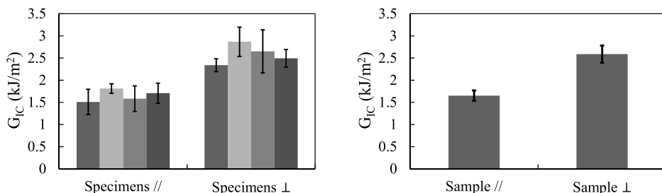
Fig. 9. Left) Average toughness values for the different specimens with standard deviation. Right) Average toughness values for the different samples with standard deviation.
