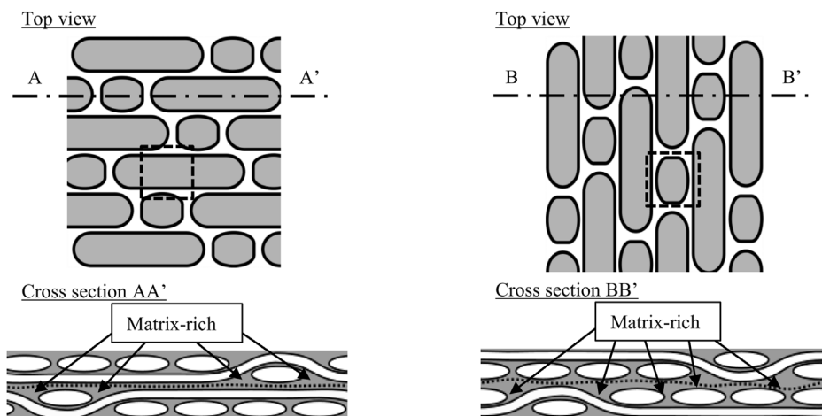
Fig. 16. Left) Represent a parallel (//) specimen, Right) represent a perpendicular (⊥) specimen. The square boxes represent the areas where the high magnification SEM image was taken. The dotted lines in the bottom image (cross-section) represent the crack propagation path.
