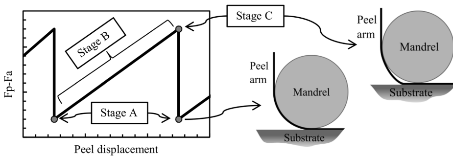
Fig. 13. Schematic illustration of the peel arm behaviour during testing.
