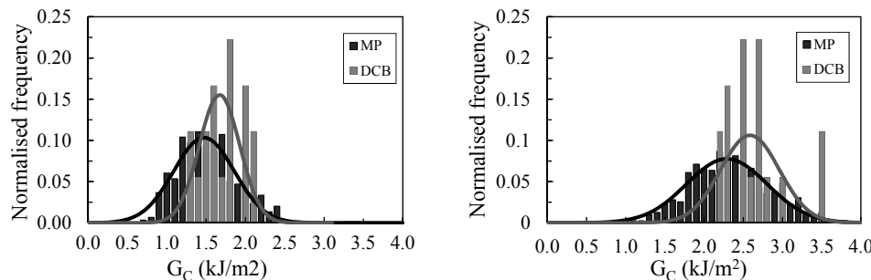
Fig. 22. Normalised frequency in function of interlaminar fracture toughness for double cantilever beam (DCB) and mandrel peel test (MP). Left) parallel sample. Right) Perpendicular sample.
