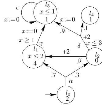
Figure 2. Example P^2TA with one clock x
