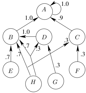
Figure 6. SPS for the symbolic graph in Figure 5
