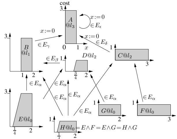
Figure 5. Symbolic graph for P^2TA of Figure 2
