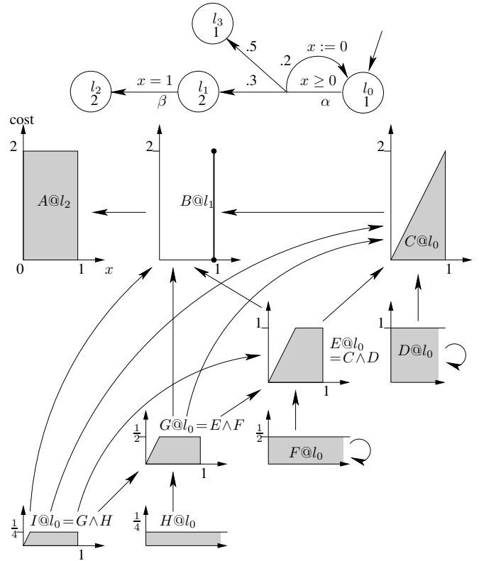
Figure 7. Example P 2 TA [7] and its infinite symbolic graph up to iteration 5
