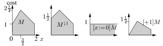
Figure 4. Predecessor operators applied on M .
