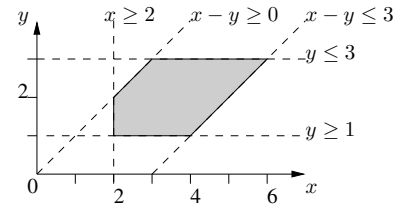
Figure 1. Example zone with clocks x and y
