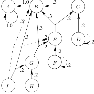
Figure 8. SPS for symbolic graph in Figure 7 Some non-optimal edges are omitted to improve readability.
