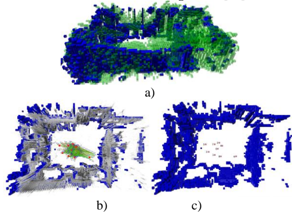
Fig. 10. 3D occupancy grid representation. a) 3D occupancy map defined by blue occupied voxels and green free voxels. b) Top view of a point cloud superimposed on the derived voxels. c) Occupied voxels are shown in blue [67].
