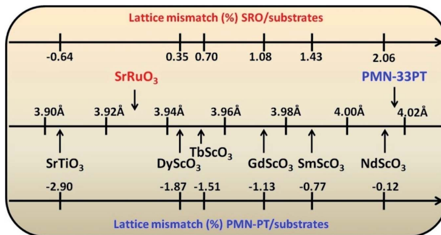
Fig. 3 The diagram presents a comparison of the pseudocubic lattice constants and the lattice mismatch between STO and \text{ReScO}_3 (Dy–Nd) substrates and PMN–33PT and SRO.
