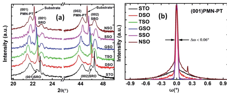
Fig. 4 (a) \theta – 2\theta XRD patterns of PMN–33PT/SRO/(STO and \text{ReScO}_3 ) heterostructures and (b) the rocking curves of PMN–33PT layers around (001) diffraction peak.
