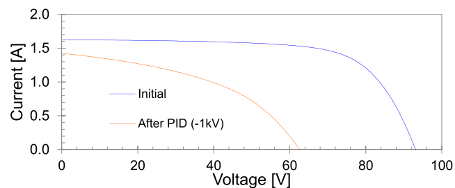
FIGURE 1 I – V curves of the module before and after the bias application of –1000 V for 48 h in a climate chamber at 85°C and 85% relative humidity (RH) [Colour figure can be viewed at wileyonlinelibrary.com ]
