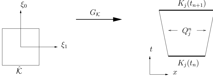
Fig. 2. Mapping G_K between the master element \hat{K} and the space-time element K_j^n with boundaries \partial K_j^n = K_j(t_n^+) \cup K_j(t_{n+1}^-) \cup Q_j^n .
