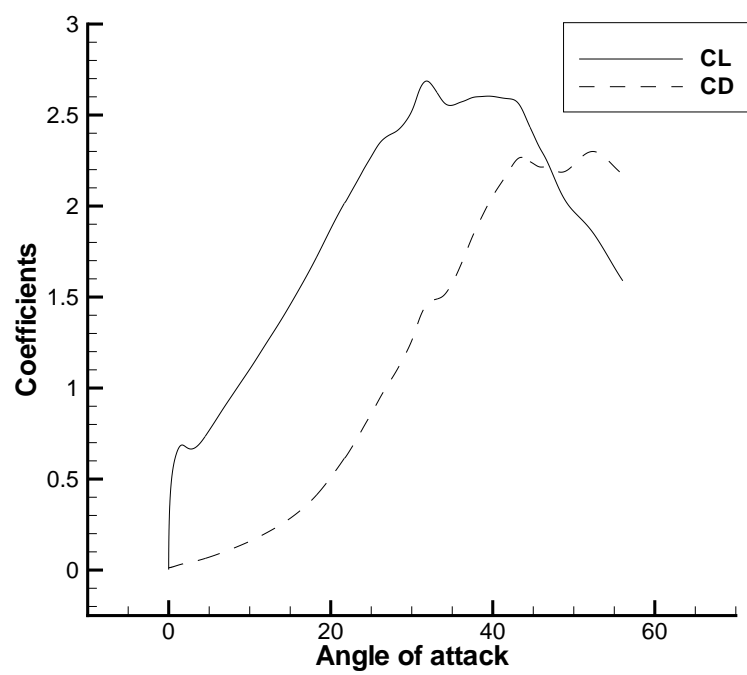
Fig. 9. The lift and drag coefficients.
