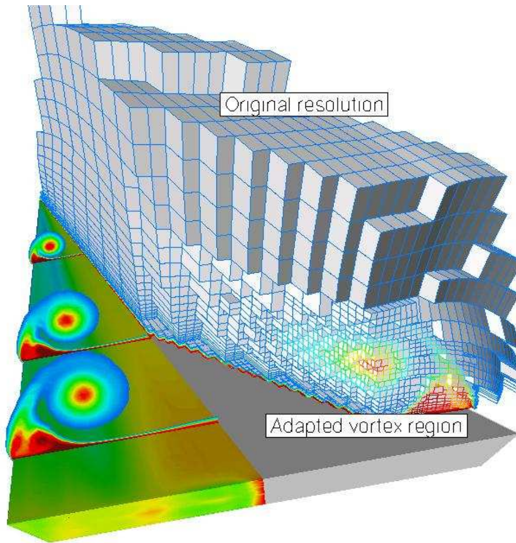
Fig. 13. Impression of the vorticity based mesh adaptation.
