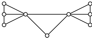
Figure 5: The graph Z in the proof of Theorem 5.3.
