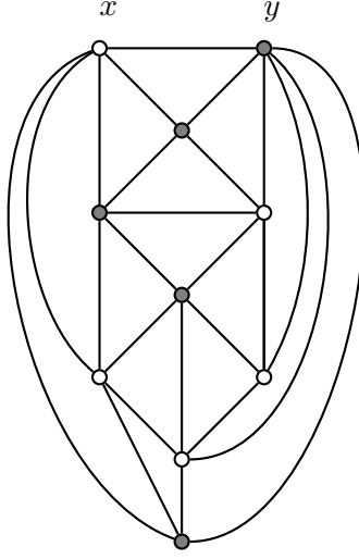
Figure 3: A gadget for the forbidden set \mathcal{F}_{345} in Theorem 4.3.
