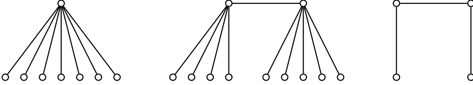
Figure 1: The graph K_{1,7} and the double-stars X_{4,5} and X_{1,1} .
