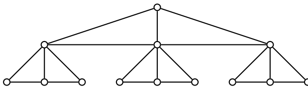
Figure 4: Example for the graph Y_3 .
