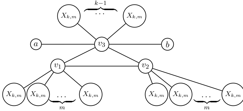
Figure 2: An equalizer for the double-star X_{k,m} .
