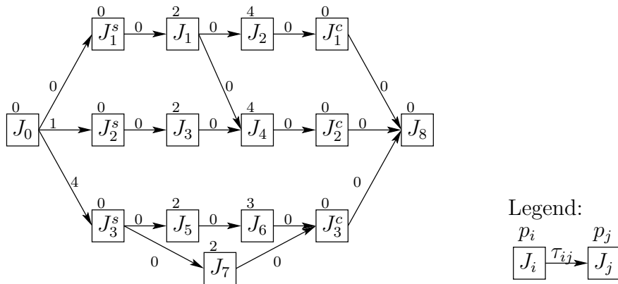
Figure 1: Example project: Activity-on-Arrow representation.
