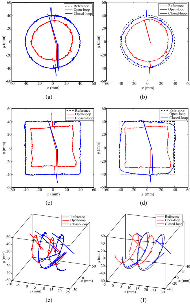
Fig. 7. Trajectory tracking with manipulator tip for a circle (2D), a square (2D) and a helix (3D). Open-loop results (red) are compared with closed-loop results (blue). (a) Circle (40 mm radius), speed is 2 deg/s. (b) Circle (40 mm radius), speed is 30 deg/s. (c) Square (80 mm edges), speed is 5 mm/s. (d) Square (80 mm edges), speed is 20 mm/s. (e) Helix, (40 mm radius), speed is 2 deg/s. (f) Helix, (40 mm radius), speed is 30 deg/s. Please refer to the attached video that demonstrates the results of the trajectory tracking experiments using our testbed.
