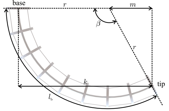
Fig. 4. Top view of the manipulator (with length l_b ) as it bends with a constant radius of curvature ( r ). The angle \beta is related to the radius of curvature by: \beta = l_b/r . The deflection of the tip with respect to the base is given by k .
