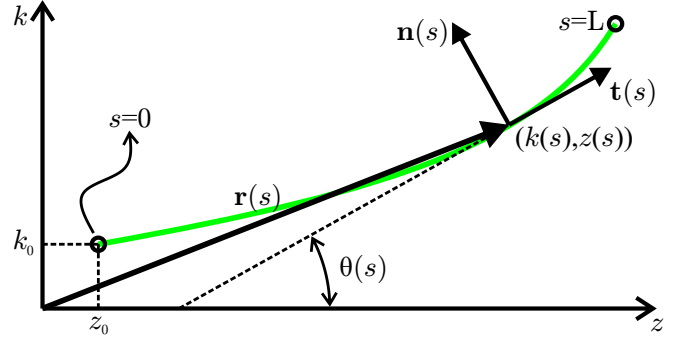
Fig. 2. A planar curve ( \mathbf{r}(s) ) is parametrized by the arc length ( s ). The slope with respect to the z -axis is denoted by \theta(s) . The Frenet-Serret vectors are also shown: The tangent vector ( \mathbf{t}(s) ) and normal vector ( \mathbf{n}(s) ).
