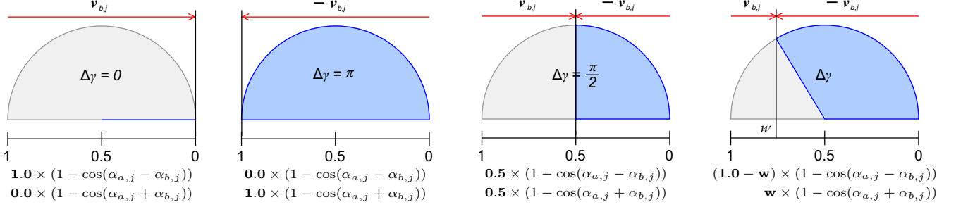
Figure 2: The proposed cosine-based distance for 3D rotations, with varying angles between rotation axes (denoted by \Delta\gamma ). Our distance is expressed as a weighted sum of the 2D cosine-based distance, and its counterpart with flipped angle \alpha_{b,j} .
