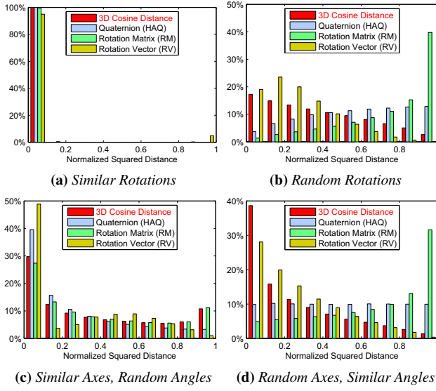
Figure 3: Histograms of squared distances d(\mathbf{r}_{a,j}, \mathbf{r}_{b,j})^2 for (a) similar and (b) uniformly distributed random rotations, rotations with (c) similar axes and (d) similar angles, each resulting from 10^5 3D rotation comparisons. Random rotations are taken from the left Haar measure on SO(3) [9, 24].
