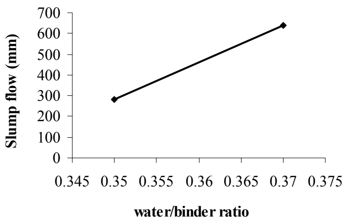
Figure 15 Slump flow Mixes 1 and 2 versus w/b ratio.
