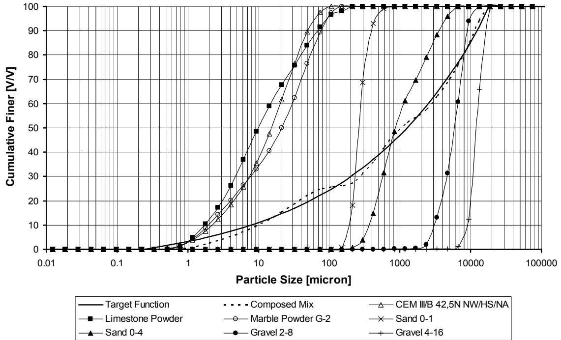
Figure 7 PSD of a mix (dashed line) composed with the help of the new design concept. The target function (solid line) as well as the PSDs of all applied materials are given too (measured with Malvern 2000 and a \sqrt{2} sieve set).
