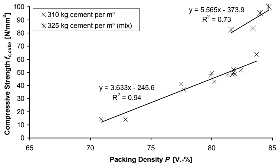
Figure 11 Compressive strength versus packing density for tested preliminary mixes with cement content of 310 kg and 325 kg per m 3 concrete, respectively.
