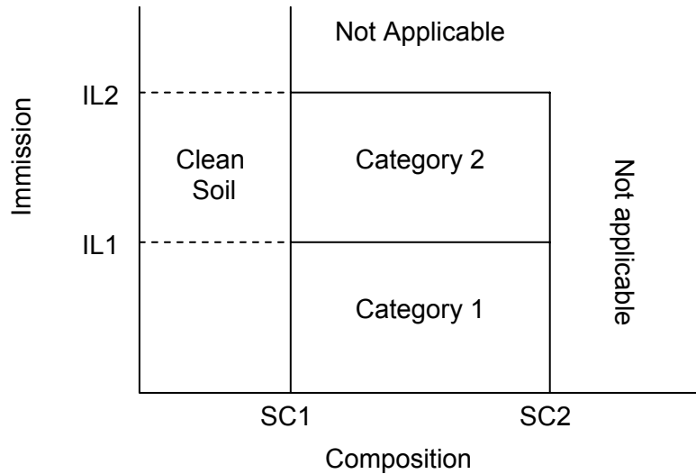
Figure 16 Classification of soil for the applicability as building material (SC = standard composition, IL = immission level).
