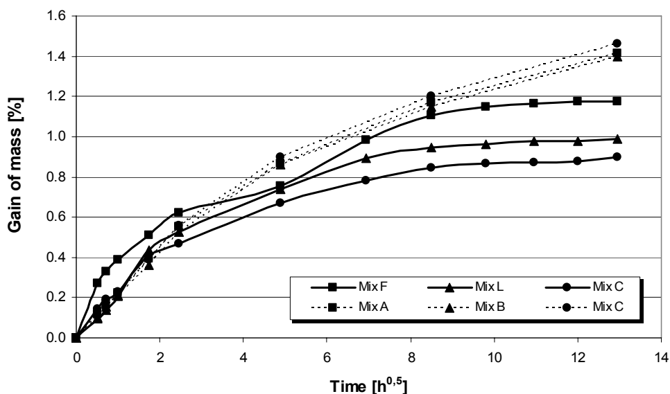
Figure 9 Capillary water absorption of three different mixes (F = fly ash, L = limestone, C = only cement as powder) composed using D_{\max} = 32 mm, compared with 3 SCC mixes with D_{\max} = 16 mm (A, B and C from Brouwers and Radix (2005)).
