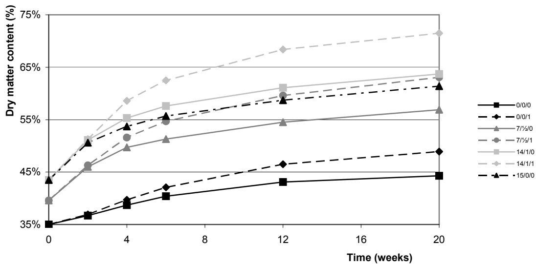
Figure 17 Actual dry matter content (%) versus time (weeks) based on drying at 105 °C.
