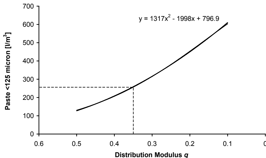
Figure 12 Computed paste content (particles < 125 \mu\text{m} plus water) per \text{m}^3 concrete for a given water/ powder ratio (w/p) of 0.35; D_{\text{max}} = 18.9 \text{ mm} , D_{\text{min}} = 12.3 \text{ nm} .
