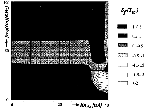
Figure 4: The tps-graph when the impact of the model is lowered to 75\text{K}\Omega . Compare fig. 2.
