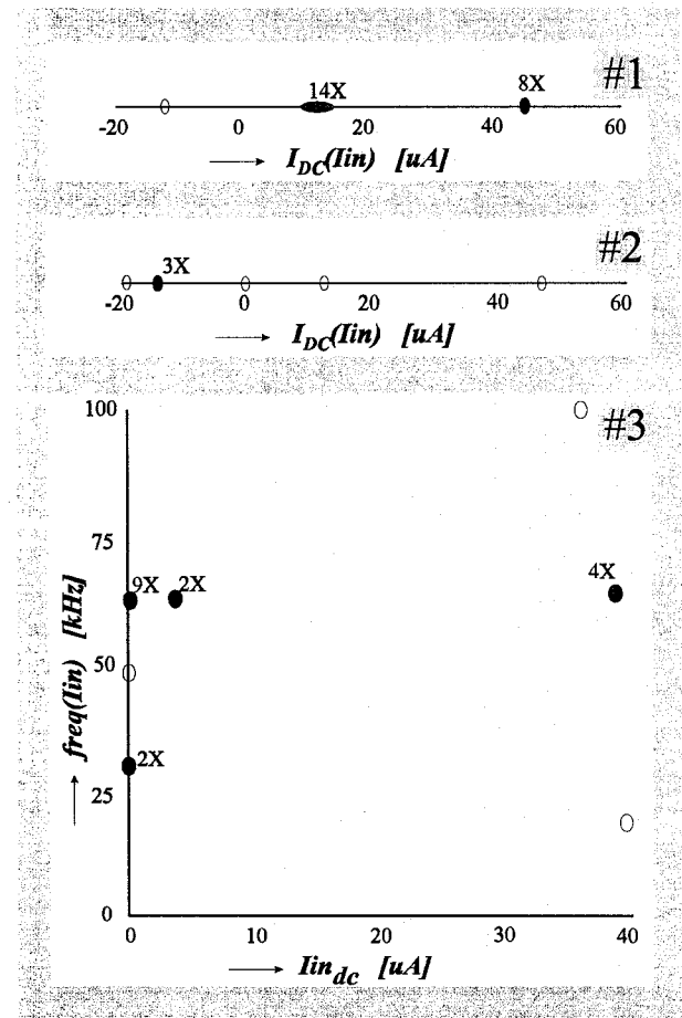
Figure 8: Optimal test parameter values resulting from test configurations #1, #2 and #3.
