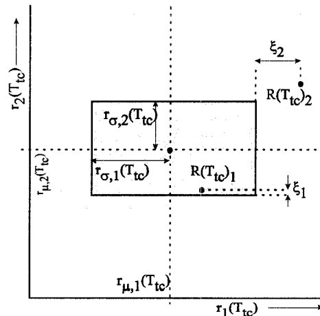
Figure 5: Visualization of 2 return values, depicted with according (gray) tolerance box and nominal values.
