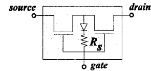
Figure 7: The pinhole fault type model
