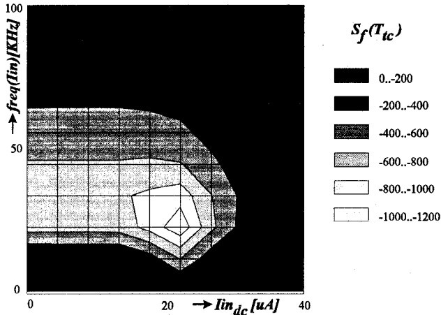
Figure 2: A tps-graph for a resistive short modeled by a 10\text{K}\Omega bridge resistance, describing a THD measurement for IV-converter macros.
