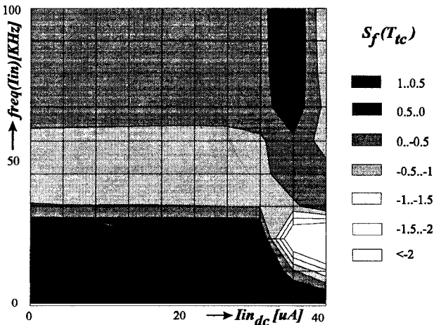
Figure 3: The tps-graph when the impact of the model is lowered to 34\text{K}\Omega . Compare fig. 2.
