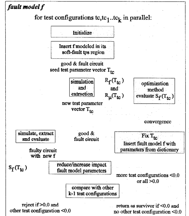
Figure 6: Scheme for the test generation for an element in the fault dictionary.
