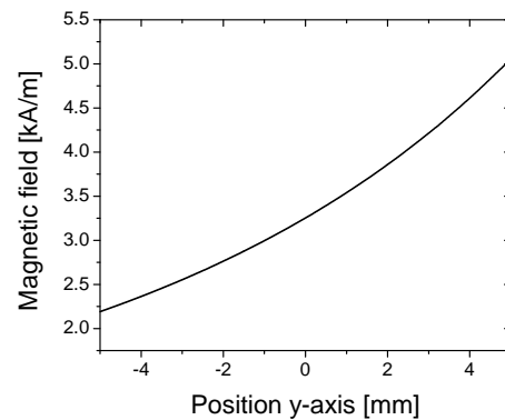
(b) The y-component of the magnetic field produced by a single coil in the liquid container
