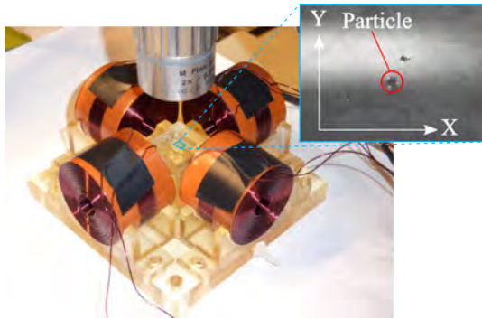
Figure 2: Image of the magnetic setup with the four coils and the microscope. The inset shows the camera picture with a small cluster of particles
