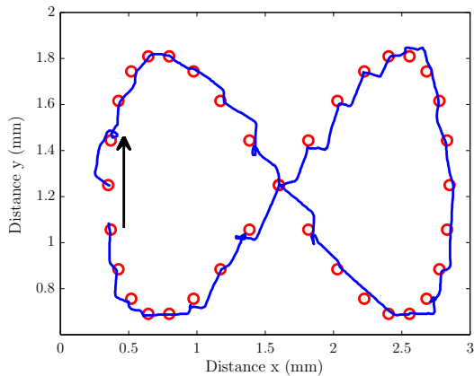
Figure 5: Comparison the setpoints given to the control software (red dots) and the path of the particles cluster (blue line)
