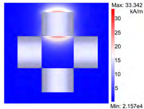
(a) Magnetic field produced by a single coil
