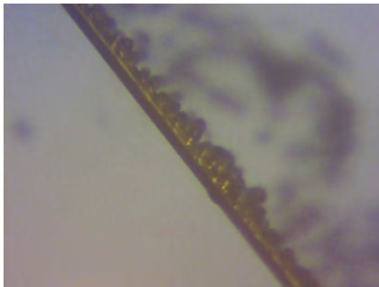
Figure 6: Piece of gold bondwire with a layer of sputtered platinum in hydrogen peroxide solution where only bubbles are formed on the platinum side
