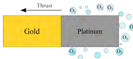
Figure 1: Schematic view of a gold and platinum rod where the platinum side catalyses the hydrogen peroxide and oxygen bubbles are formed
