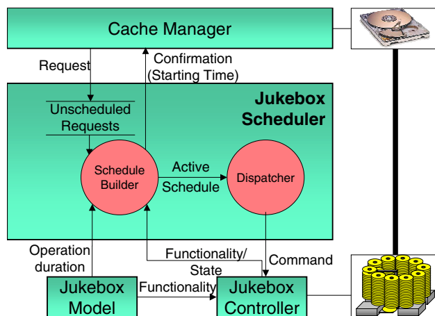
Figure 2. Jukebox-scheduler architecture.
