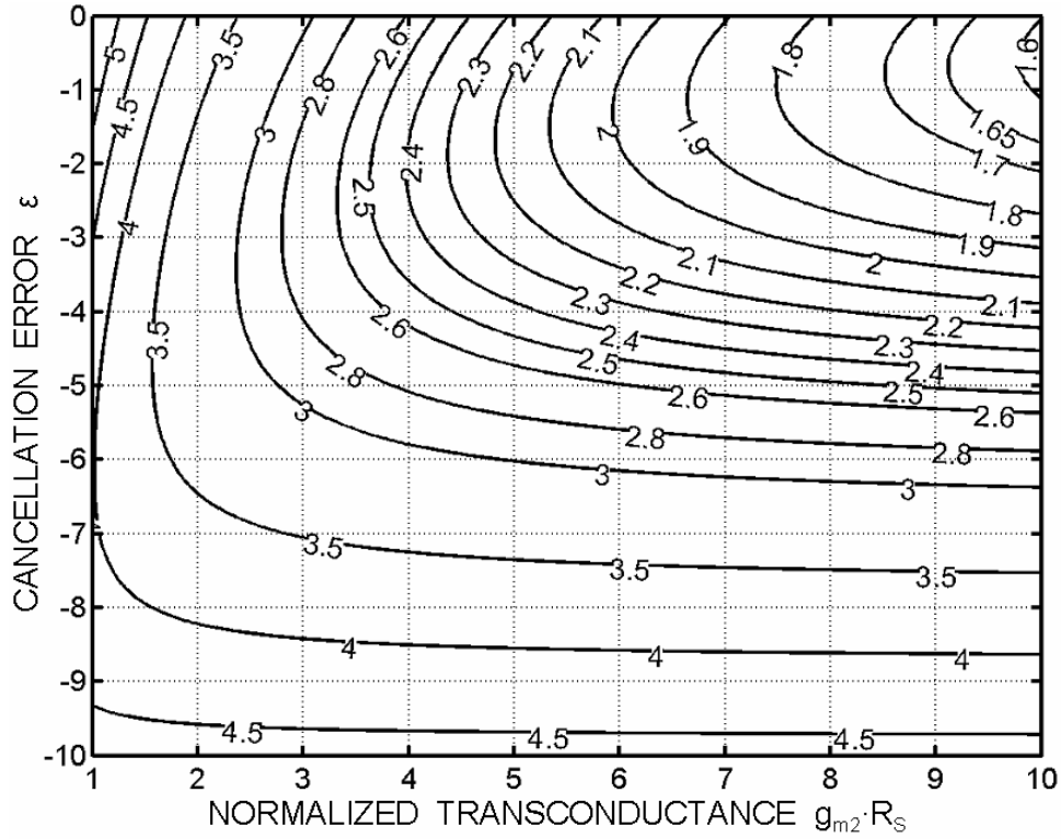
Figure 5.4: Contour lines of the LNA noise figure NF(\epsilon, g_{m2}R_S) for n=0 and R_o=\infty .
