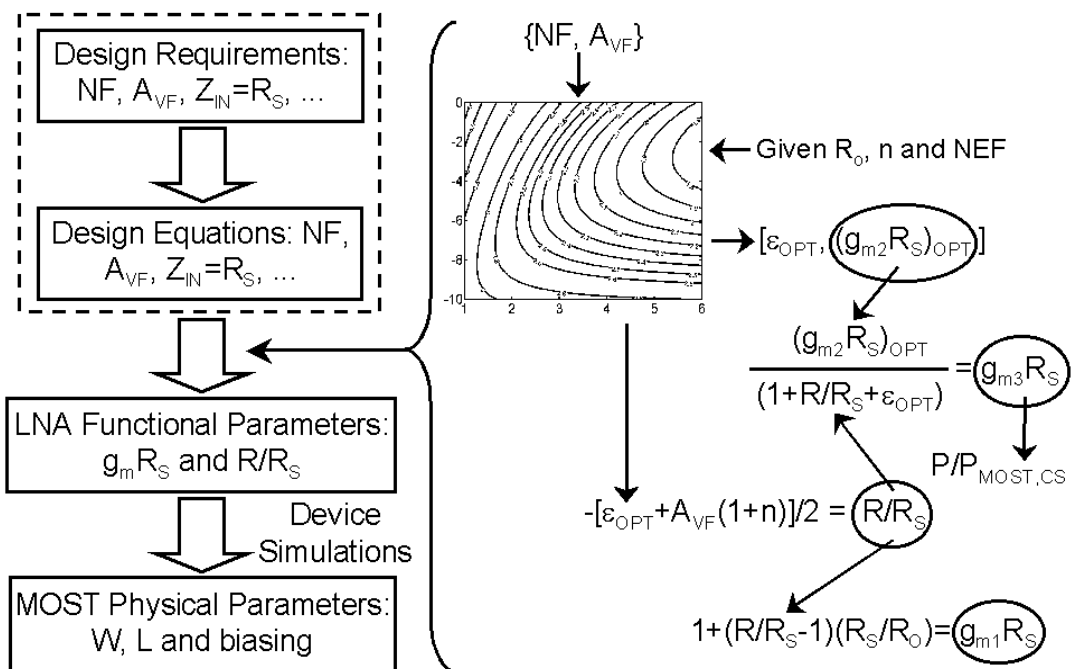
Figure 5.12: Description of the LNA design procedure.
