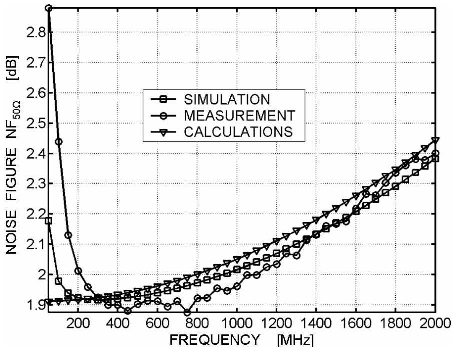
Figure 6.7: Measured and simulated NF versus frequency.
