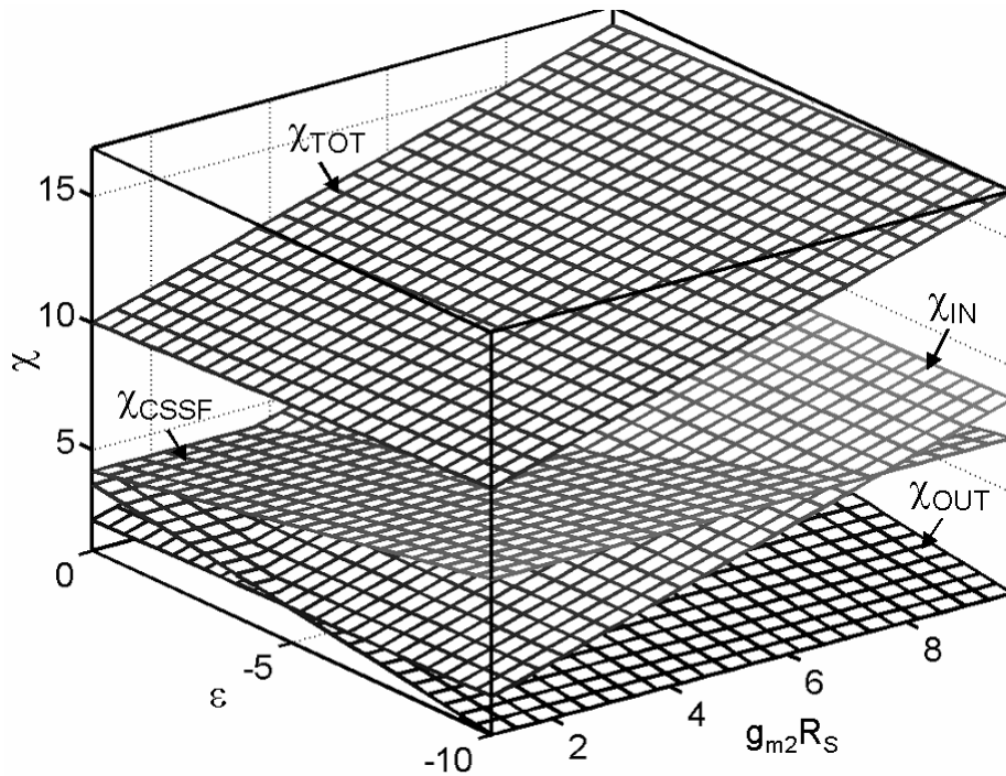
Figure 5.10: \chi versus (\varepsilon, g_{m2}R_S) for A_{VF}=-10 , n=0.2 , NEF=1.5 , R_O=1\text{K}\Omega , L_{\text{min}}=0.25\mu\text{m} , \alpha_{\text{ov},n}=0.2 , \alpha_{\text{ov},p}=0.5 , \alpha_{j,n}=0.32 , \alpha_{j,p}=0.28 and \alpha_{np}=2.5 .
