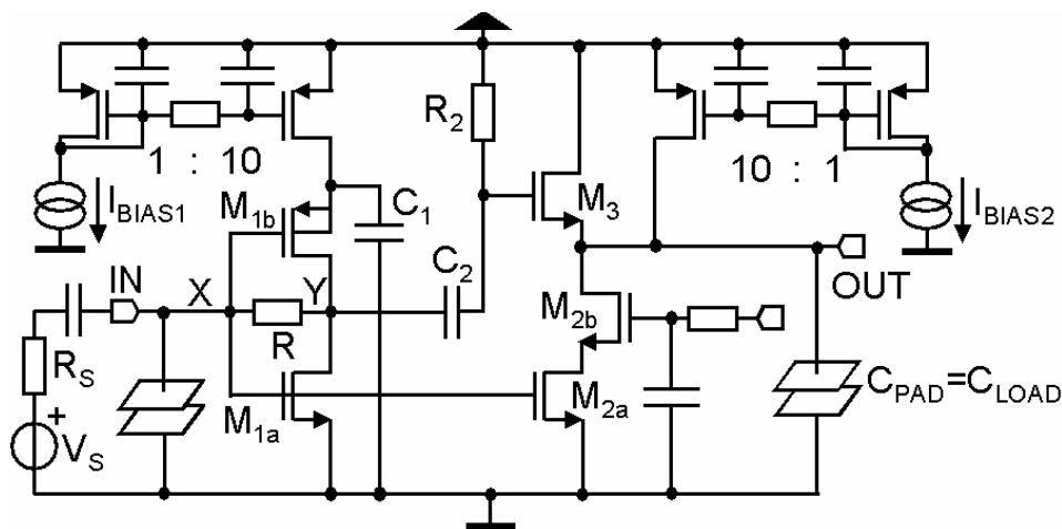
Figure 5.1: Schematic of the selected wide-band LNA circuit.
