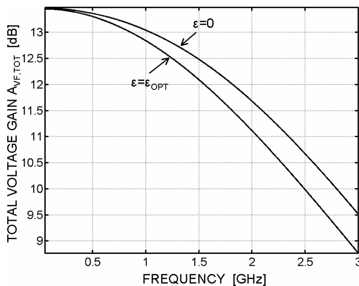
Figure 5.17: Total gain, A_{\text{VF,TOT}} versus frequency for \epsilon=0 and \epsilon=\epsilon_{\text{OPT}}=-4.5 .
