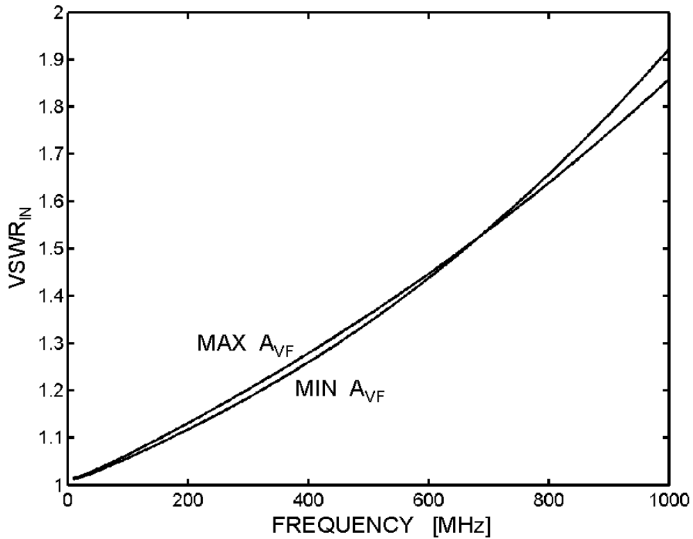
Figure 3.10: Simulated input voltage standing wave ratio versus frequency.
