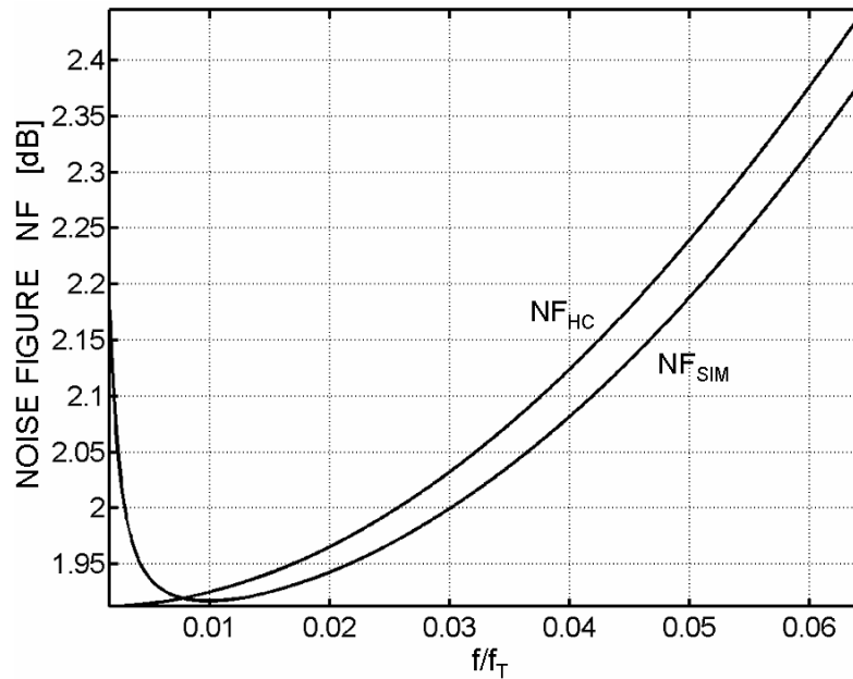
Figure 5.20: Simulated \text{NF}_{\text{SIM}} and calculated \text{NF}_{\text{HC}} versus f/f_T ( f_T = 31\text{GHz} @ V_{GS} - V_{T0} = 250\text{mV} ) for \epsilon = \epsilon_{\text{OPT}} = -4 .
