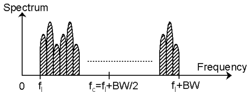
Figure 1.2: A wide-band signal spectrum spanning a bandwidth from f_i to f_i+BW with center frequency, f_i+BW/2 , such that the ratio BW/(f_i+BW/2) can be as large as 2 (i.e. for BW/2 \gg f_i ).
