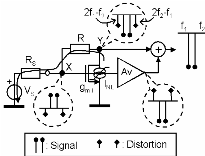
Figure 4.33: Cancellation of 3 rd order intermodulation terms sketched in the frequency domain.
