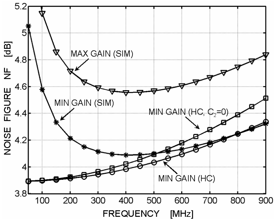
Figure 3.12: NF for R_S=75\Omega versus frequency (HC=Calculations; SIM=Simulations).
