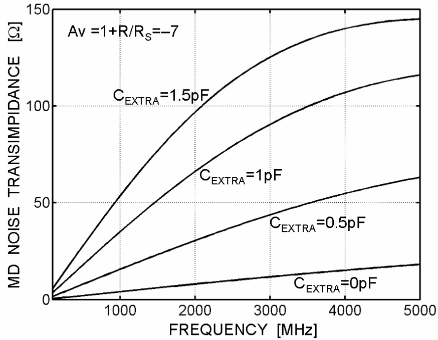
Figure 4.39: Simulated matching-device noise trans-impedance versus frequency for different values of C_{EXTRA} .
