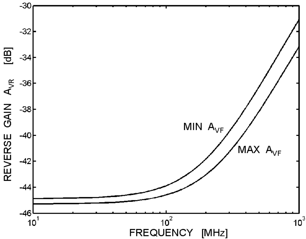
Figure 3.11: Simulated reverse gain A_{VR}=20\log_{10}(V_{IN}/V_{OUT}) versus frequency.
