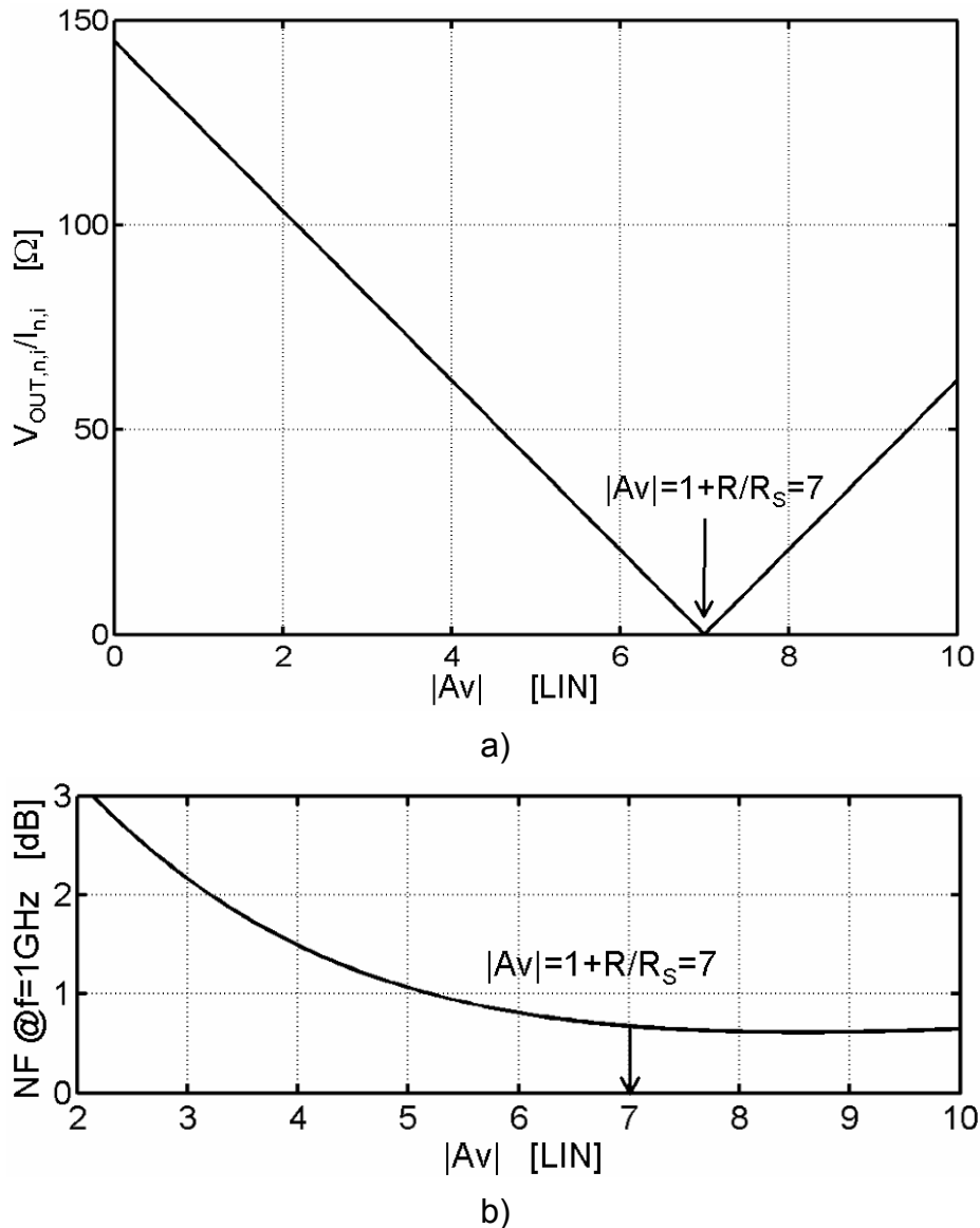
Figure 4.21: (a) Simulated transfer function from the noise current I_{n,i} to the output versus the gain |Av| @1GHz and (b) Simulated noise figure versus the gain |Av| @1GHz.
