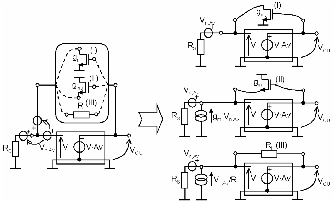
Figure 4.7: Noise models used to calculate contribution to F of amplifier Av (biasing not shown).
