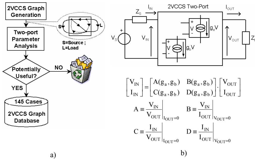
Figure 2.2: a) Flow chart describing the steps leading to the generation of the 2VCCS database b) A 2VCCS two-port circuit described by \{A, B, C, D\} parameters. The latter are a function of the transconductances g_a and g_b of the 2 VCCSs (i.e. VCCS a and VCCS b ).
