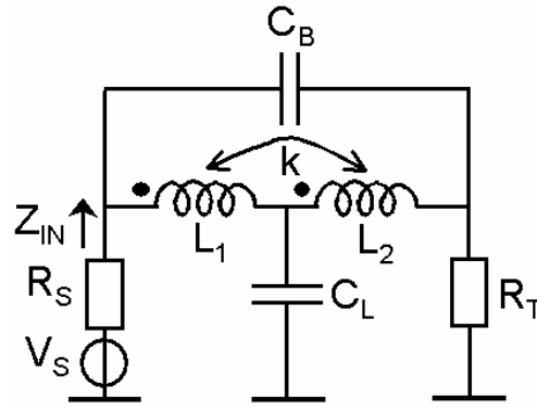
Figure 4.46: Bridged T-coil network.
