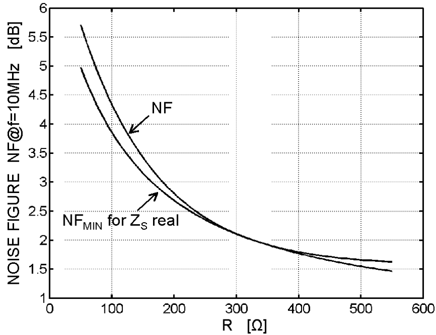
Figure 5.14: Noise figure (NF) and minimum NF_{MIN} versus R for large C_1 and C_2 .
