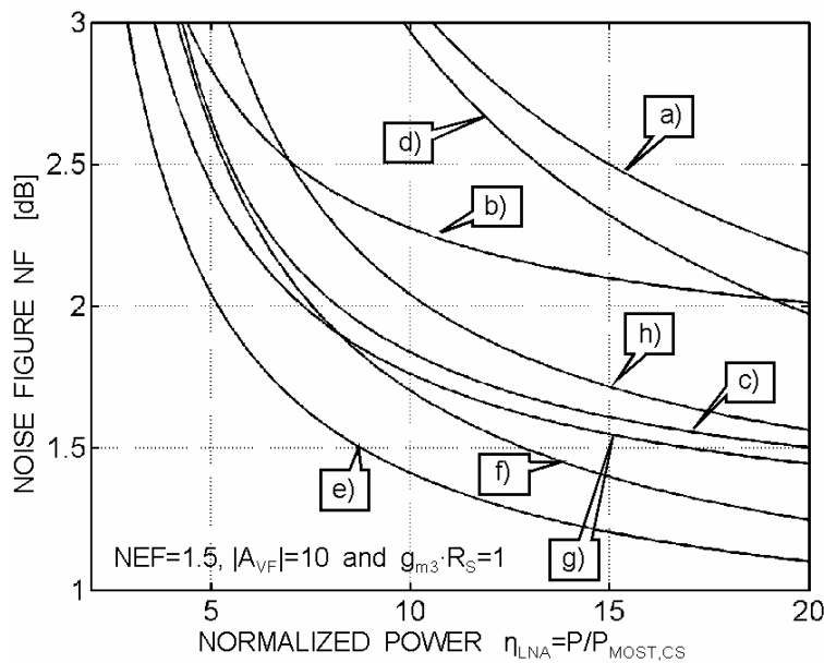
Figure 4.23: NF versus \eta_{\text{LNA}} for Z_{\text{IN}}=R_S and constant A_{\text{VF}} ( \delta=0.3 ).
