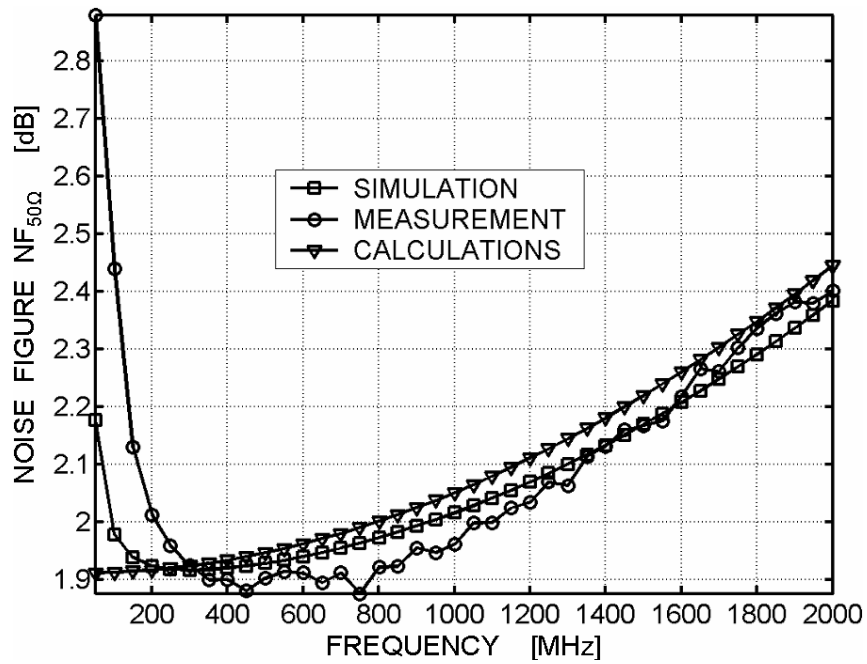
Figure 5.26: Measured, simulated and calculated NF versus frequency.
