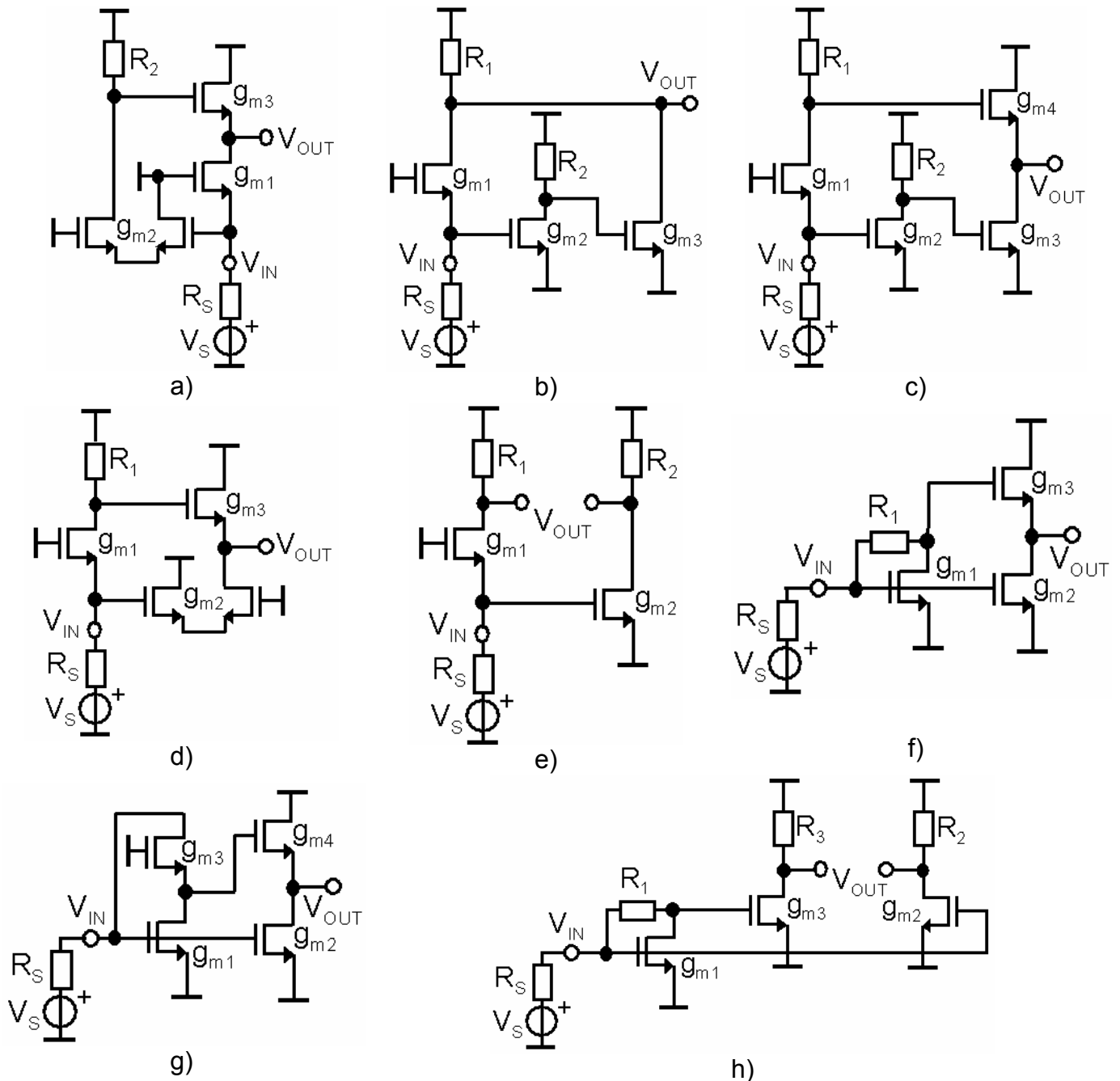
Figure 4.16: Alternative implementations of a noise-cancelling amplifier (biasing not shown).
