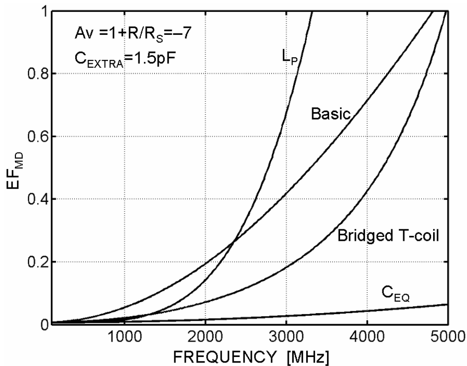
Figure 4.49: Simulated EF_{MD} versus frequency for different frequency-compensation techniques.
