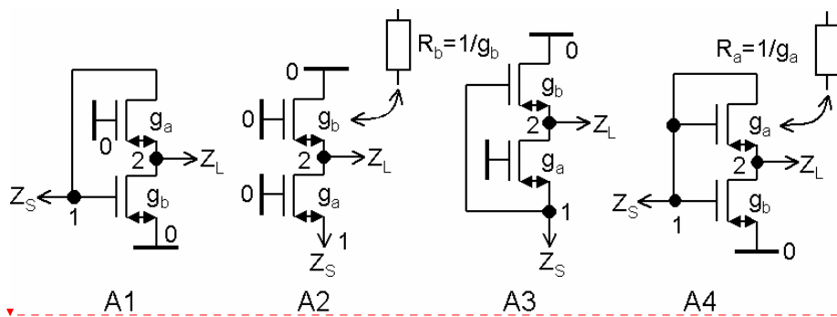
Figure 2.11: Implementation of A1-A4 with MOSFETs or resistors (biasing not shown).
