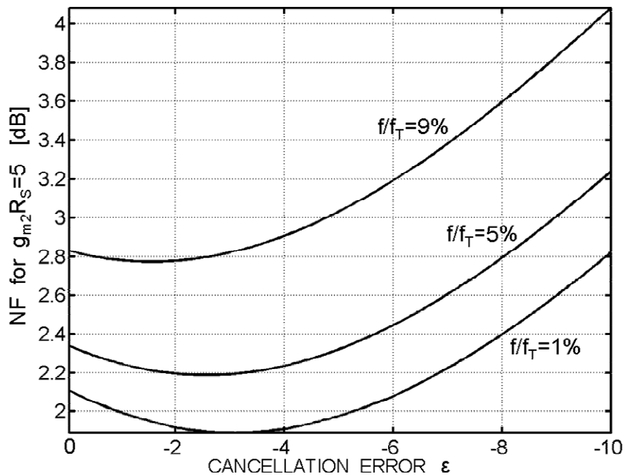
Figure 5.9: NF versus \epsilon=0 for g_{m2}R_S=5 and f/f_T = 0.01, 0.05 and 0.09 .
