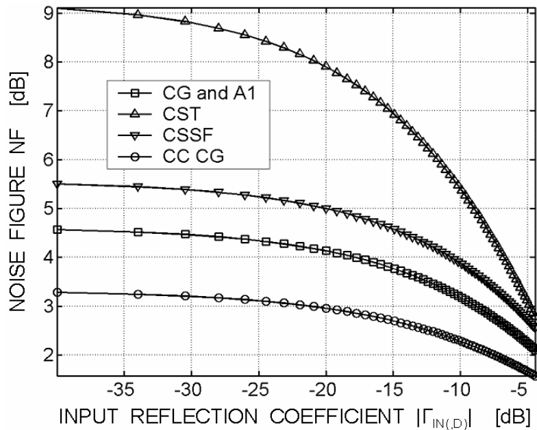
Figure 4.5: NF versus |\Gamma_{IN(D)}| for |A_{VF,TOT}|=5 ( NEF=1.5 ).
