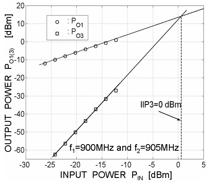
Figure 5.28: Measured (on-PCB) IIP3.
