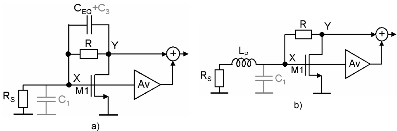
Figure 4.45: Methods to improve noise cancelling: noise equalization (a) and peaking coil (b).
