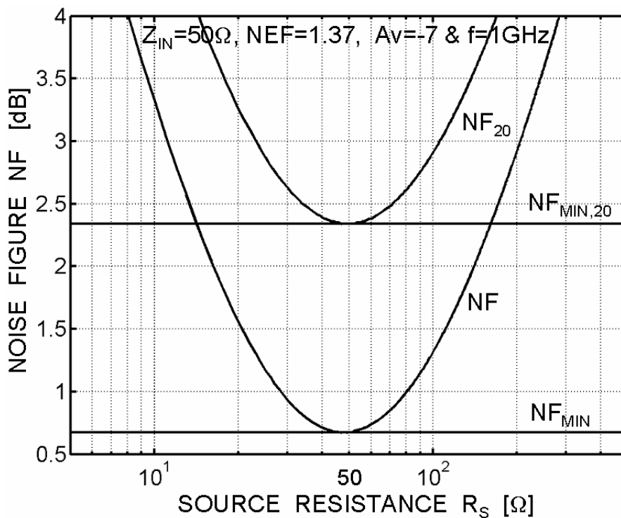
Figure 4.31: Simulated NF ( NF_{20} ) and NF_{MIN} ( NF_{MIN,20} ) versus R_S for the LNA in figure 4.20c (MOS model 9) for a noiseless (noisy) amplifier “Av”. The matching-stage provides R_{IN} \approx 50\Omega for V_{GS} - V_{T0} \approx 250mV . R = 300\Omega renders a voltage gain ( =V_Y/V_X ) of 12.8dB for the matching stage.
