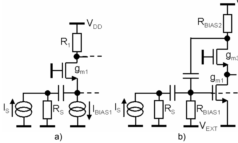
Figure B.1: Biasing of the matching stage used in the LNAs of figure 4.16.
