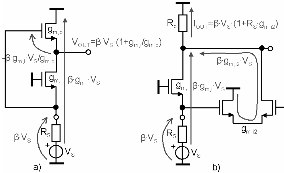
Figure 4.12: Addition of signals for the LNAs in figure 4.11.
