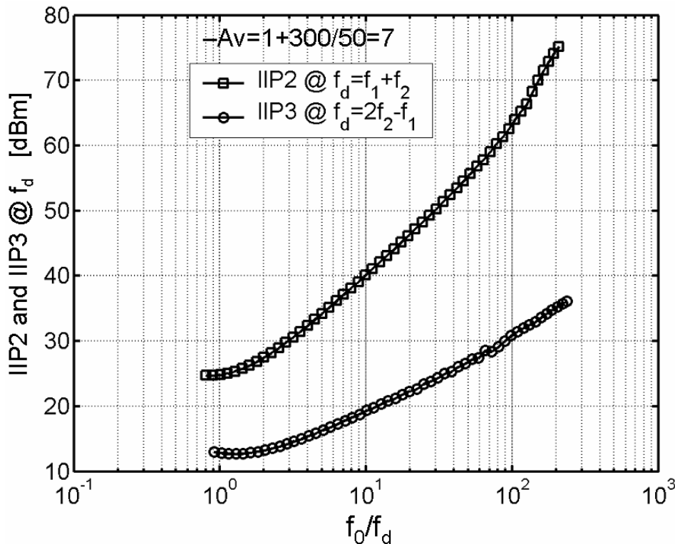
Figure 4.44: Simulated IIP2 and IIP3 versus f_0/f_d .
