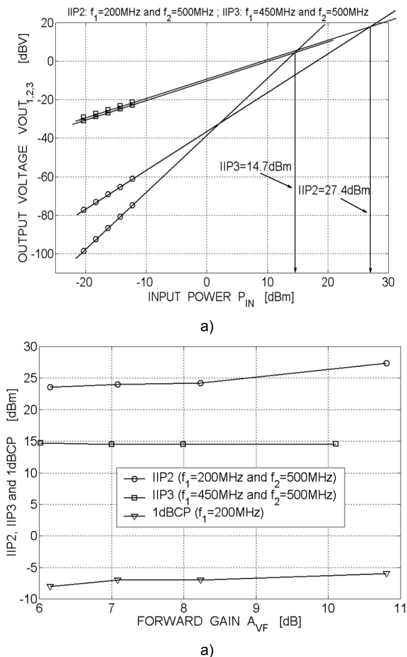
Figure 3.17: Measured IIP2 and IIP3 at maximum gain (a) and IIP2, IIP3 and 1dBCP vs. gain (b).
