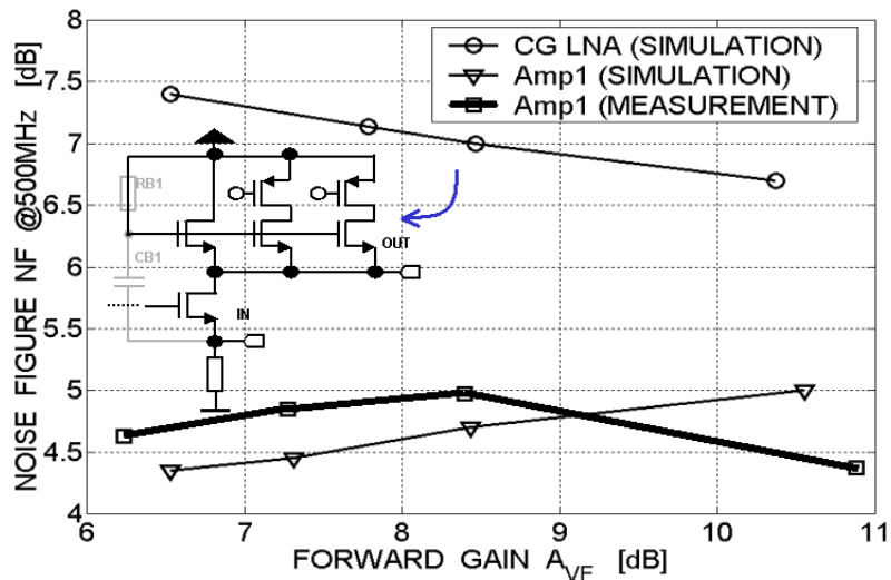
Figure 6.3: NF_{50@500MHz} versus A_{VF} for the LNA of figure 6.2 and a CG amplifier derived from it (see text).
