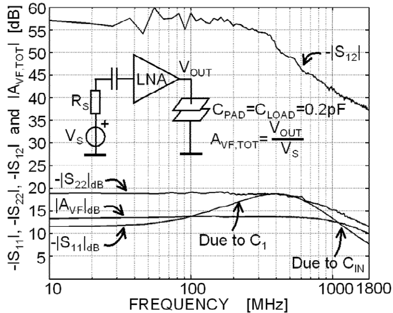
Figure 5.24: Measured (on-wafer) S_{11} , S_{22} , S_{12} and A_{VF,TOT} versus frequency.
