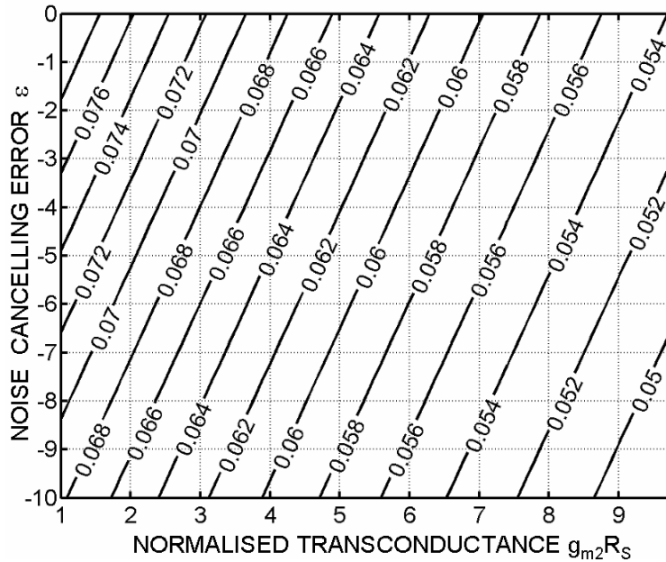
Figure 5.11: Contours of f_{3dB}/f_T versus (\varepsilon, g_{m2}R_S) for A_{VF}=-10 , n=0.2 , NEF=1.5 , R_O=1K\Omega , L_{min}=0.25\mu m , \alpha_{ov,n}=0.2 , \alpha_{ov,p}=0.5 , \alpha_{jn}=0.32 , \alpha_{jp}=0.28 and \alpha_{np}=2.5 .
