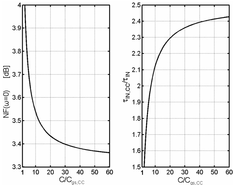
Figure 4.4: a) NF(\omega=0) versus C/C_{gs,CC} and (b) \tau_{IN,CC}/\tau_{IN} versus C/C_{gs,CC} ( NEF=1.5 , A_{VF,TOT,D}(\omega=0)=5 and C_p=C_{gs,CC} ).
