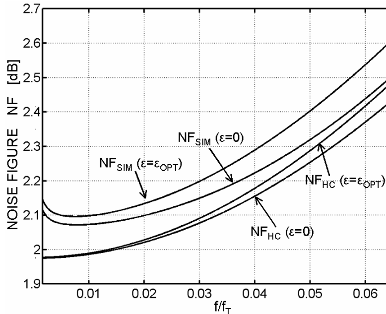
Figure 5.16: Simulated \text{NF}_{\text{SIM}} and calculated \text{NF}_{\text{HC}} versus f/f_T ( f_T=31\text{GHz} @ V_{\text{GS}}-V_{\text{T0}}=250\text{mV} ): \epsilon=0 and \epsilon=\epsilon_{\text{OPT}}=-4.5 .
