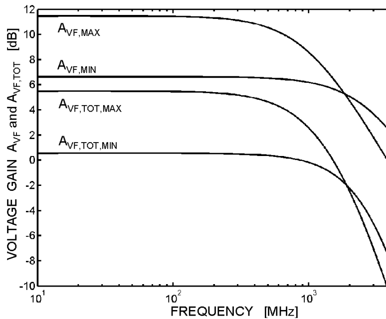
Figure 3.8: Simulated amplifier voltage gains A_{VF} and A_{VF,TOT} .
