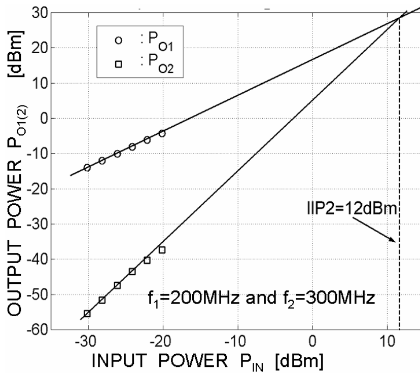
Figure 5.27: Measured (on-PCB) IIP2.
