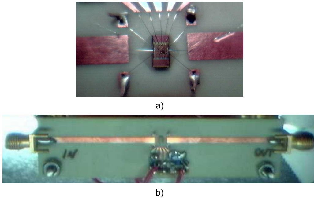
Figure 5.25: Photos of the PCB set-up used to measure noise figure and distortion.
