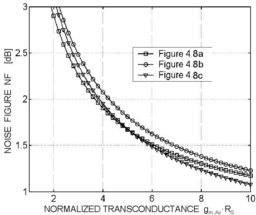
Figure 4.9: NF versus g_{m,Av}R_S for Z_{IN}=R_S , A_v=-10 and NEF=1.5 .
