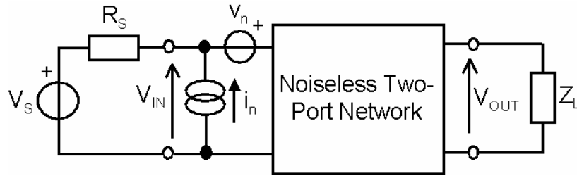
Figure 4.30: Two-port noise model: “ i_n ” and “ v_n ” are the equivalent input noise current and voltage.
