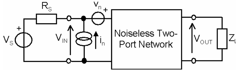
Figure C.1: Two-port circuit noise model.
