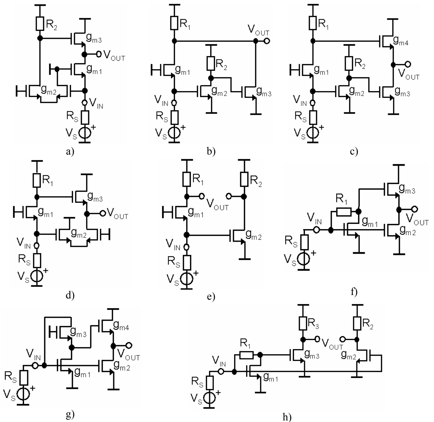
Figure 6.5: systematically generated alternative noise-cancelling amplifier (biasing not shown).
