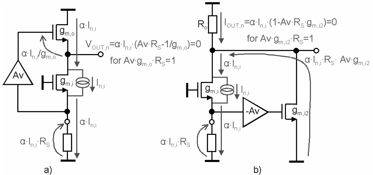
Figure 4.13: Improved noise-cancelling LNAs (biasing not shown).
