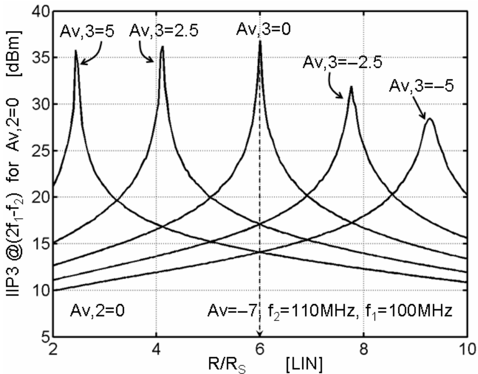
Figure 4.36: Simulated IIP3 versus R/R_S for different values of A_{v,3} and A_{v,2} = 0 (MOS model 9) for the amplifier in figure 4.33. The matching-stage provides R_{IN} \approx R_S = 50\Omega for V_{GS} - V_{T0} \approx 250\text{mV} while R = 300\Omega renders a voltage gain ( =V_Y/V_X ) of 12.8dB for the matching stage.
