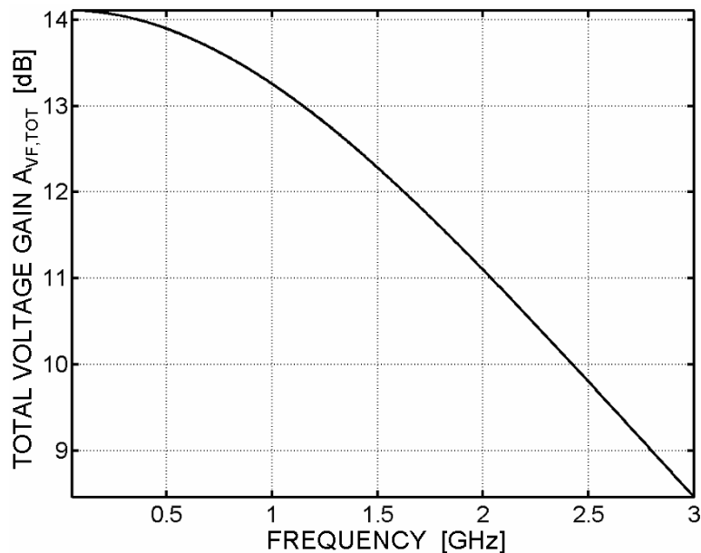
Figure 5.21: Total voltage gain A_{V,F,TOT} versus frequency (50MHz to 3GHz) for \epsilon = \epsilon_{\text{OPT}} = -4 .
