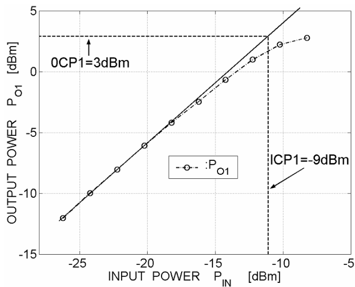
Figure 5.29: Measured (on-PCB) ICP1dB.
