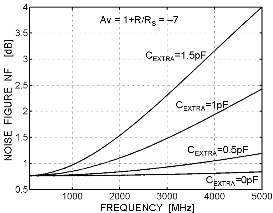
Figure 4.40: Simulated NF versus frequency for different values of C_{EXTRA} .
