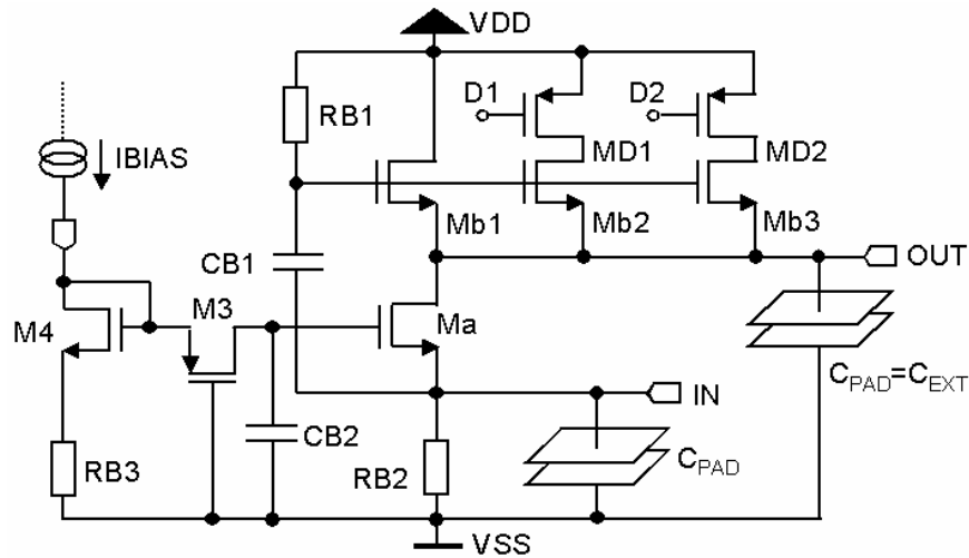
Figure 3.5: Wide-band LNA based on A3 (bond pad is used as load).
