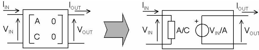
Figure 2.7: A two-port circuit with parameters \{A, 0, C, 0\} .
