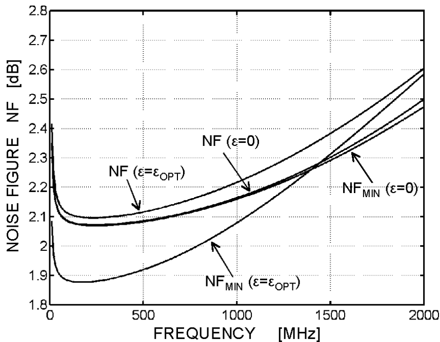
Figure 5.15: Simulated NF and NF_{MIN} versus frequency (10MHz to 2GHz) for: \epsilon=0 and \epsilon=\epsilon_{OPT}=-4.5 .
