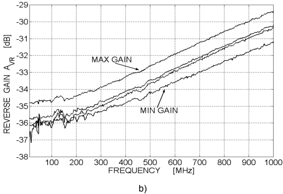
Figure 3.14: Measured A_{VF} (a) and A_{VR} (b) versus frequency for different settings.
