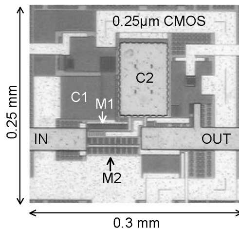
Figure 5.23: Die-photo of the wide-band 0.25 \mu\text{m} CMOS LNA.
