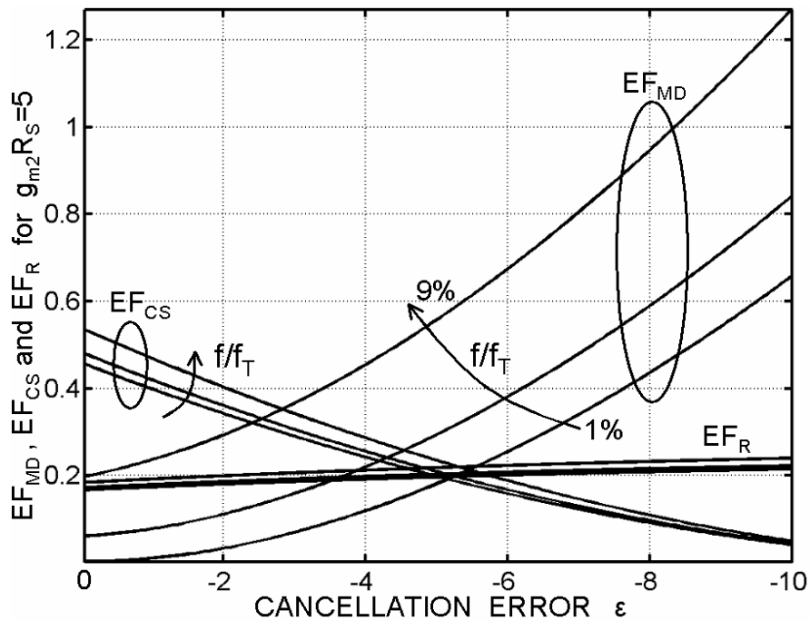
Figure 5.8: EF's versus \epsilon=0 for g_{m2}R_S=5 and f/f_T = 0.01, 0.05 and 0.09 .
