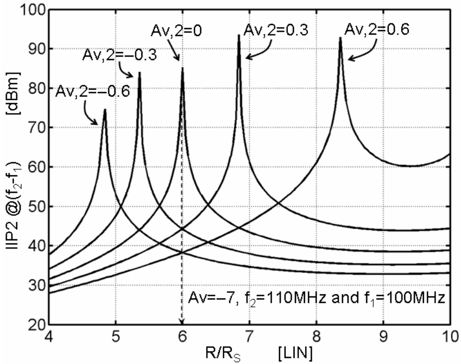
Figure 4.35: Simulated IIP2 versus R/R_S for different values of A_{v,2} (MOS model 9) for the amplifier in figure 4.33. The matching-stage provides R_{IN} \approx R_S = 50\Omega for V_{GS} - V_{T0} \approx 250\text{mV} while R = 300\Omega renders a voltage gain ( =V_Y/V_X ) of 12.8dB for the matching stage.
