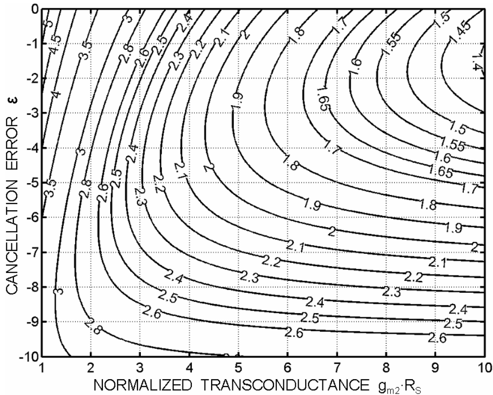
Figure 5.3: Contour lines of the LNA noise figure NF(\varepsilon, g_{m2}R_S) for R_O = 1K\Omega and n = 0.2 .
