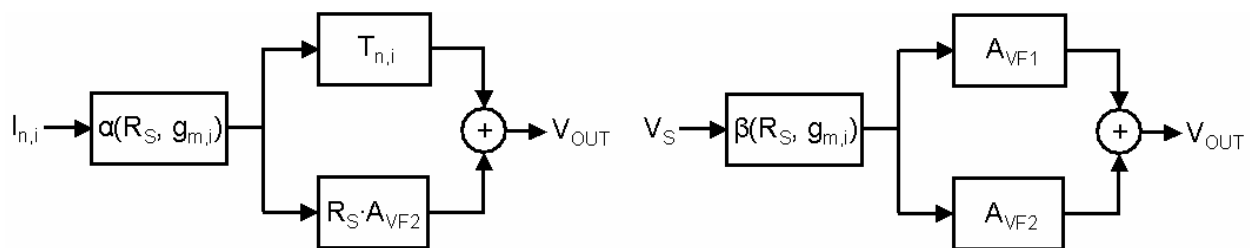
Figure 4.27: Feed-forward representation of the noise and signal transfer function.
