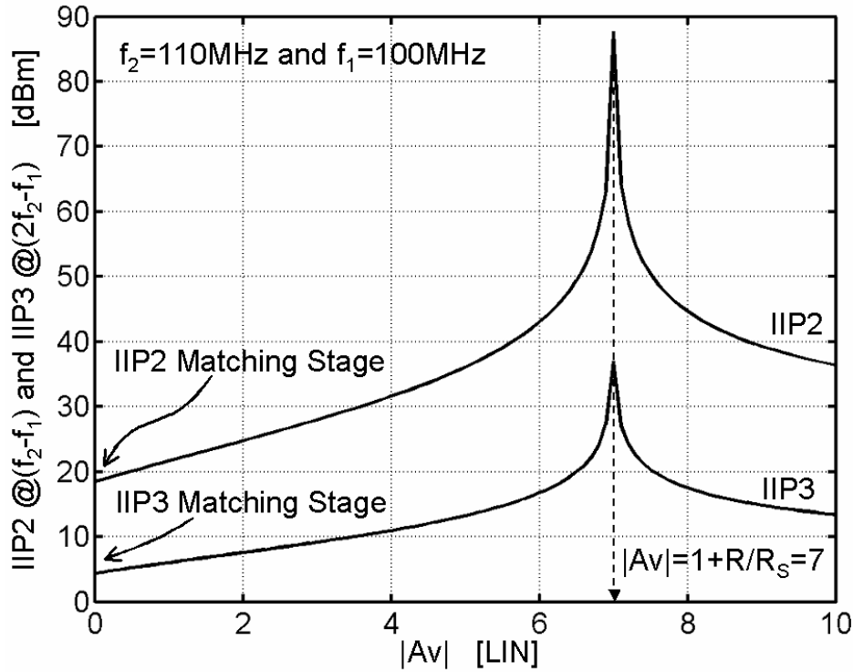
Figure 4.34: Simulated IIP2 and IIP3 versus |A_v| for the amplifier in figure 4.32 (MOS model 9). The matching-stage provides R_{IN} \approx R_S = 50\Omega for V_{GS} - V_{T0} \approx 250\text{mV} while R = 300\Omega renders a gain ( V_Y/V_X ) of 12.8dB for the matching stage.
