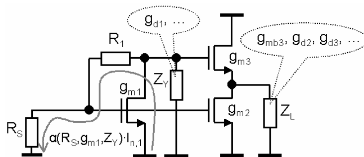
Figure 4.28: Effect of Z_Y and Z_L on noise cancelling for the amplifier in figure 4.16f.
