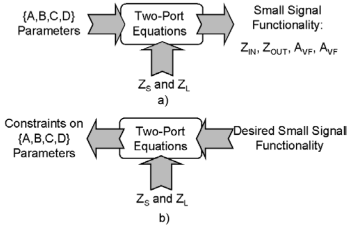
Figure 2.4: a) \{A, B, C, D\} parameters plus Z_S and Z_L determine the two-ports small-signal functionality. b) Graphs of 2VCCS wideband amplifiers are selected using the reverse reasoning: the desired amplifier functionality is translated into constraints on the \{A, B, C, D\} parameters upon assigned Z_S and Z_L . These constraints are the criteria to select useful graphs within the 2VCCS database.
