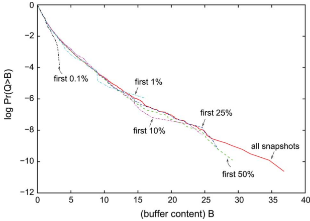
Fig. 8. Comparing \mathbb{P}(Q > B) for various trace lengths.
