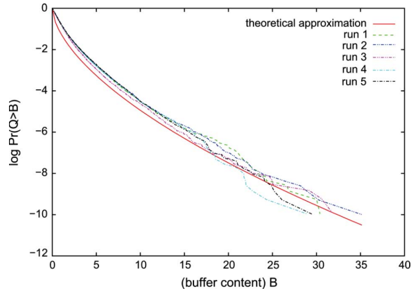
Fig. 7. \mathbb{P}(Q > B) and theoretical approximation ( H = 0.7 ).
