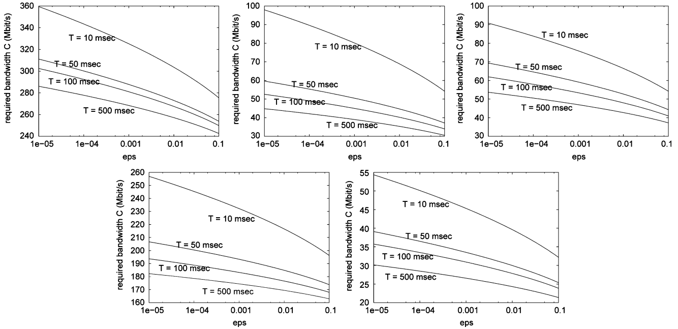
Fig. 13. Required bandwidth for other settings of T and \varepsilon for locations \{U, R, C, A, S\} .
