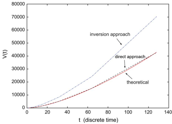
Fig. 11. Variance curves for Gaussian/non-Gaussian traffic mixture, \alpha = 0 .
