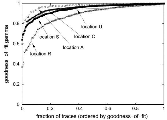
Fig. 1. Distribution of the linear correlation coefficient over all measurements.
