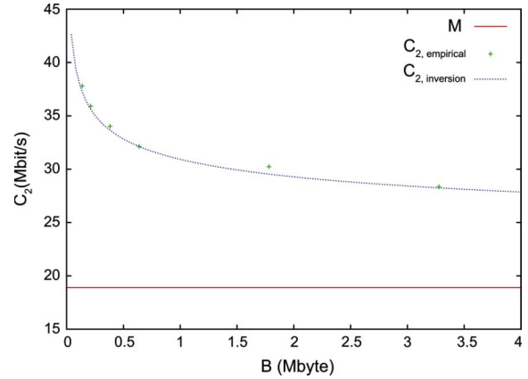
Fig. 12. Required bandwidth as a function of the buffer size B for a trace at location R. The ‘+’ are the empirical values, and the line is the curve using the estimate of V(\cdot) obtained by inversion; \varepsilon = 0.01 .
