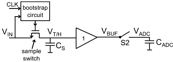
Fig. 3. Overview of 1 of the 16 T&amp;H channels; S2 is open during tracking to increase the buffer bandwidth.
