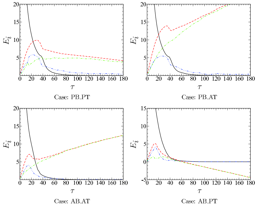
FIG. 10. Time evolution of energies E_i as function of number of rotations \tau . Kinetic energy E_k (black —), potential energy E_p (red - -), background potential energy E_b (green - · -), and available potential energy E_a (blue - · · -). The Rossby number is \epsilon = 1 .
