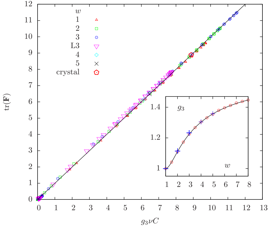
Figure 9. The trace of the fabric tensor as given by Eq. (7) for different size distributions with w given in the inset from simulations with N = 1000 (“L3” indicates a larger simulation with N = 10000 and “crystal” indicates an ordered lattice structure whereas w = 1 is a disordered, monodisperse configuration). Each data-point corresponds to one density and fabric, as averaged over the whole system, at different densities during decompression. Inset: The constant g_3 plotted as function of w from its definition (o), the analytical approximation (solid line) and the simulation data (+).
