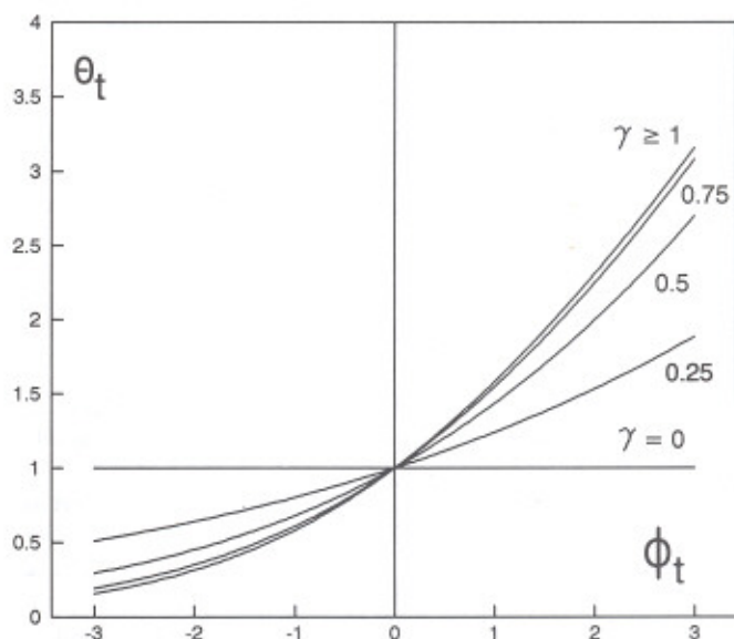
Figure 2. Thermal correction factor \Theta_t as a function of \phi_t and for various \gamma .
