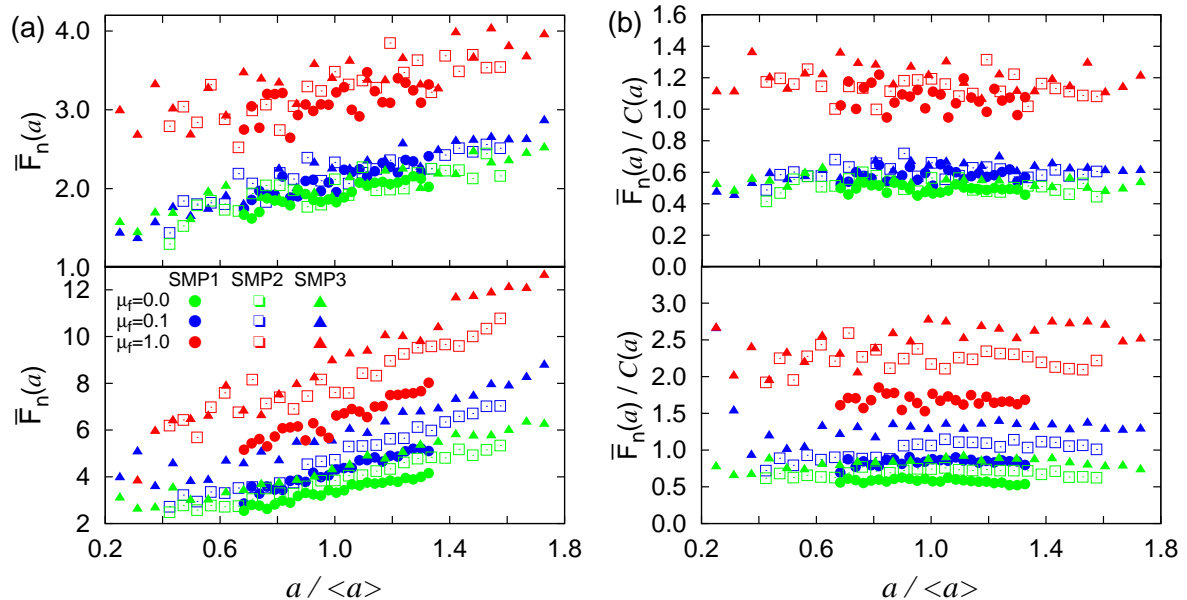
FIG. 9: (color online) (a) Normal component of the contact force \bar{F}_n(a) , averaged over all particle radii in the same bin, in terms of the particle radius a for (top) two- and (bottom) three-dimensional packings constructed with different size distribution widths and different friction coefficients \mu_f . (b) \bar{F}_n(a) scaled by the contact number C(a) for the same set of samples as in (a).
