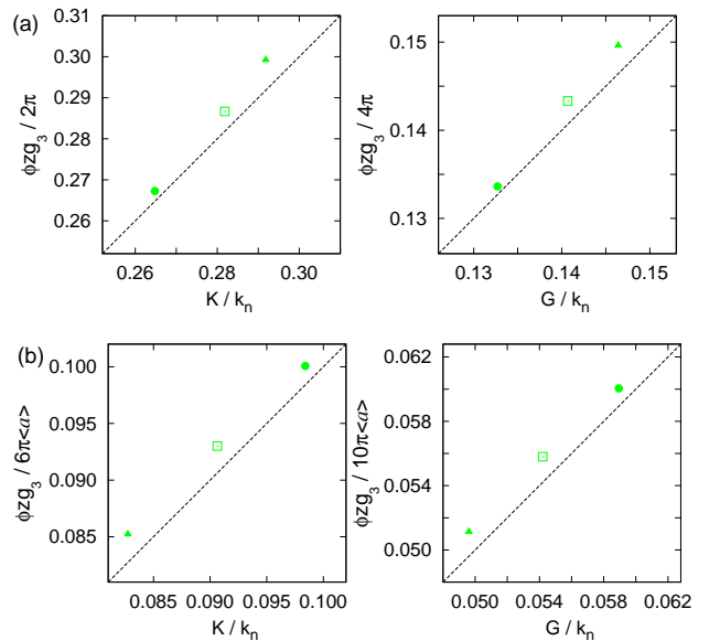
FIG. 11: (color online) The estimated values of the bulk K (left) and shear G (right) moduli according to Eqs. (42) and (43) in 3D [Eqs. (A18) and (A19)] versus the values obtained from the simulation results. Each data point corresponds to one frictionless sample and the dashed lines indicate the identity. The results are separately shown for (a) 2D and (b) 3D samples. The same symbols as in Table I are used.
