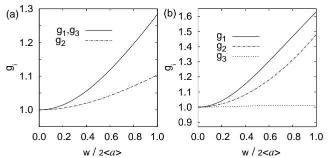
FIG. 12: The dimensionless correction factors g_i in terms of the width w of the uniform size distribution in (a) two, and (b) three dimensions. w/2\langle a \rangle = 0 corresponds to the monodisperse case.
