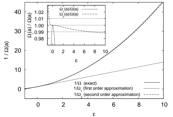
FIG. 2: 1/\Omega(a) as a function of \epsilon . The exact value (solid line) is compared with the first order (dashed line) and second order (dash-dot line) approximations. The inset shows more clearly the deviation of the approximations from the exact value.
