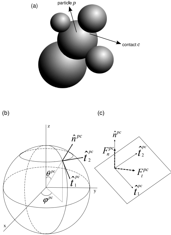
FIG. 3: (a) A typical contact c between the reference particle p and its neighboring particle. (b) The contact unit vectors \hat{n}^{pc} , \hat{t}_1^{pc} , and \hat{t}_2^{pc} . (c) The normal ( F_n^{pc} ) and tangential ( F_t^{pc} ) components of the contact force \vec{F}^{pc} .
