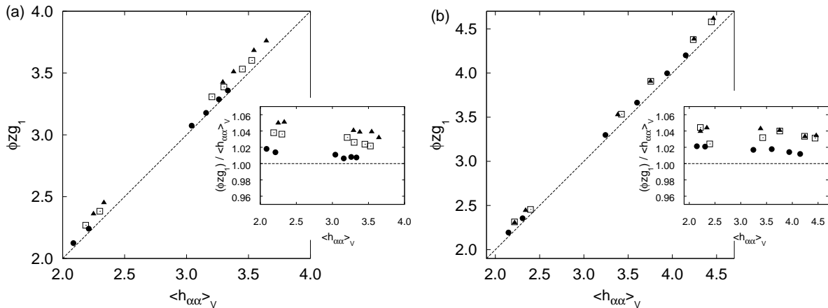
FIG. 8: The estimated value of the trace of the average fabric tensor \phi z g_1 versus the exact value \langle h_{\alpha\alpha} \rangle_V obtained from the simulations, for several (a) two- and (b) three-dimensional samples. The dashed lines indicate the identity. The insets show more precisely that the deviations increase with w , but remain less than 5% in all cases. The symbols are chosen the same as in Table I.
