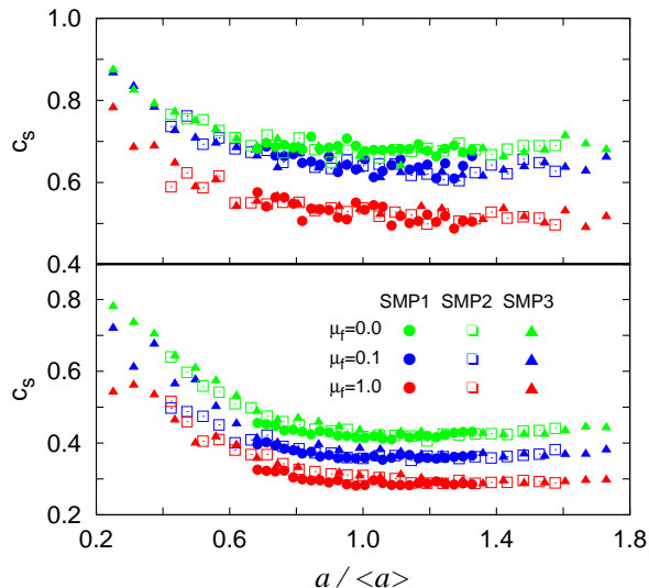
FIG. 5: (color online) Linear compacity c_s as a function of particle radius a for (top) two- and (bottom) three-dimensional packings constructed with different size distribution widths and different friction coefficients \mu_f .
