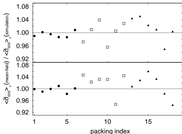
FIG. 10: The estimated value of the trace of the stress tensor using (top) Eq. (A10), and (bottom) Eq. (26) divided by \langle \sigma_{\alpha\alpha} \rangle_V obtained directly from the simulations. Each data point corresponds to a different (top) 2D or (bottom) 3D packing using symbols as in Table I.
