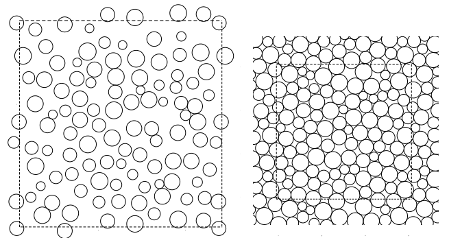
FIG. 4: Schematic of a 2D granular system subjected to a constant external pressure: (left) the initial dilute gas, and (right) the final homogeneous packing. Periodic boundaries are marked with dashed lines.
