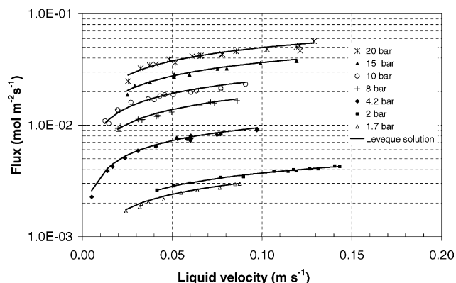
Fig. 11. Measurement of CO 2 absorption flux through the hollow fiber in propylene carbonate at elevated CO 2 pressures.
