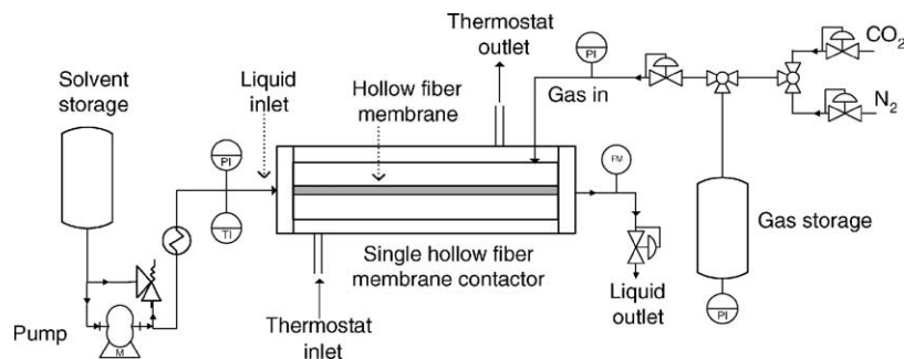
Fig. 2. Experimental setup.
