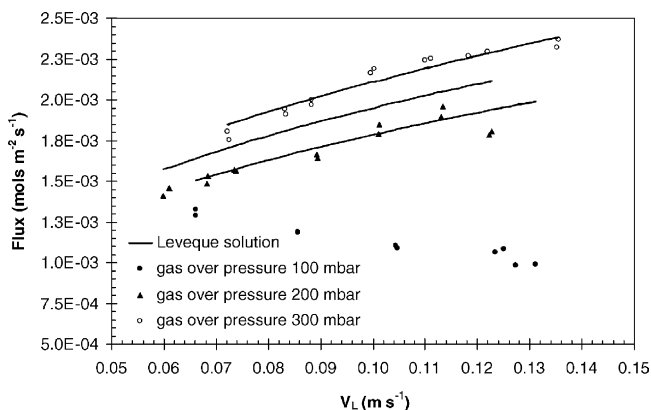
Fig. 8. Effect of gas-side over pressure on CO 2 absorption flux through the hollow fiber in propylene carbonate.
