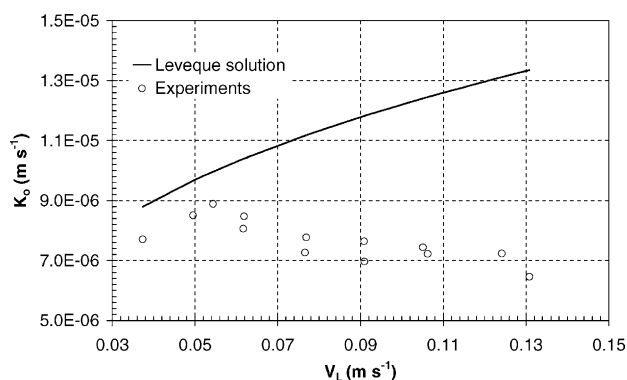
Fig. 6. Overall mass transfer coefficient for the absorption of \text{CO}_2 in propylene carbonate at atmospheric pressure after 2 weeks of operation.
