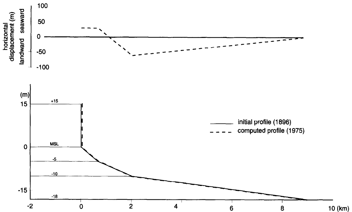
Fig. 4. Computed shoreface profile evolution 1896–1975 of the Central Holland Coast (km 70–90, see Fig. 3 for location).
