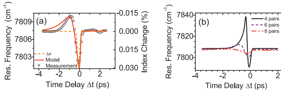
Fig. 2. (a) Measured (symbols) and calculated (red curve) resonance frequency versus time delay ( \Delta t ) between pump and probe for a GaAs/AlAs cavity ( Q = 390 \pm 60 ). The resonance frequency red-shifts due to increased refractive index only near temporal overlap ( \Delta t = 0 \pm 15 fs) of pump-probe, shown with dashed curve. (b) Calculated spectra for a GaAs/AlAs cavity that consists of 19 pairs of bottom Bragg layers, \lambda -layer, and sequentially changed number of layers on the top Bragg mirror.
