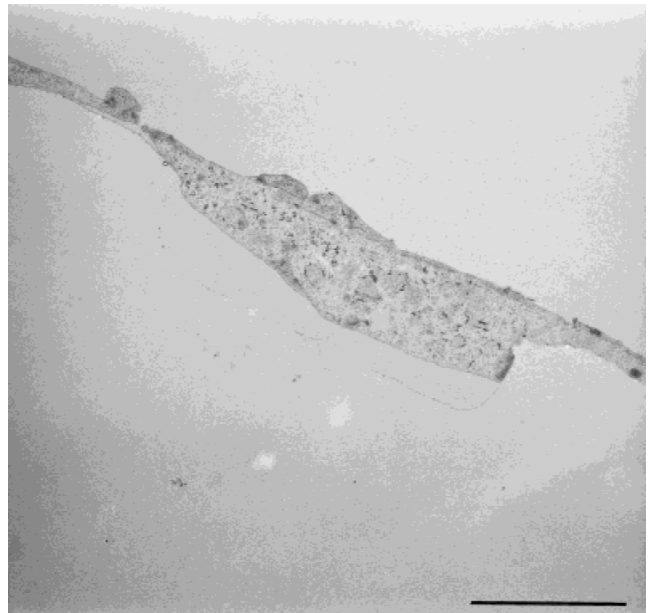
Figure 8. Transmission electron micrograph of an RDF on a TiD05 surface after 3 days of incubation (bar = 2.0 \mu\text{m} ). The cell protrudes into the groove but does not contact the bottom of the groove. Focal adhesion points can be seen on the edge of the ridge and the wall of the surface groove.
