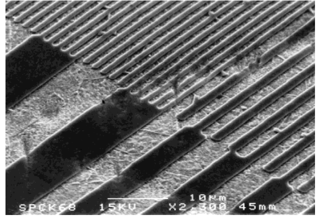
Figure 1. Scanning electron micrograph of four different microtextures on the cpTi wafer surfaces. The dents in the surface and consequential pattern damage are clearly visible. Furthermore, the protrusions on the surface edge and the difference in the roughness of the groove bottom and ridge crest can be seen.
