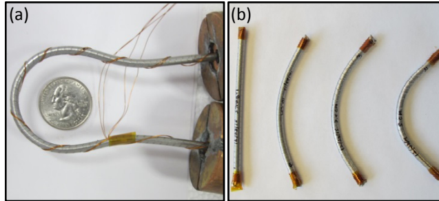
Figure 2 – (a) Section of wire 1 bent to a 3.5 cm diameter hairpin shape prior to full wire V(I) measurement. (b) 7 cm long sections of wire 1 prior to V(I) measurements on extracted tapes.
