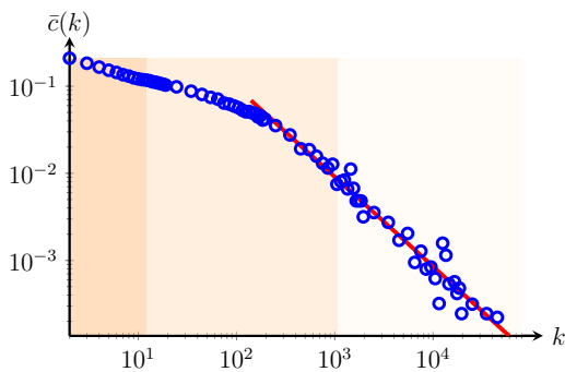
Figure 1. \bar{c}(k) for the YouTube social network
