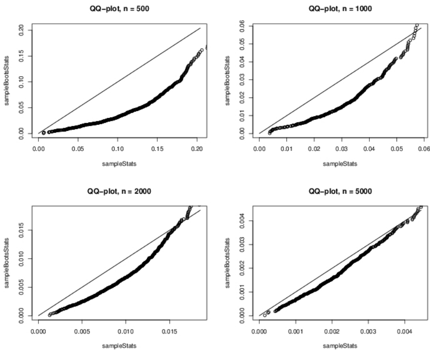
Figure 5: QQ-plot of a sample of the test statistic \bar{T}_2^C and a sample of the bootstrap test statistic (\bar{T}_2^C)^* using the non-parametric bootstrap for the gaussian copula, with different sample sizes and under \bar{T}_0^C (conditional Kendall’s tau is constant and equal to 0.5).
