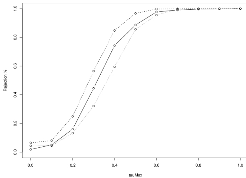
Figure 4: Rejection percentages for the statistics \bar{T}_2^C(30) as a function of \tau_{max} : we use the gaussian copula, with a conditional parameter \theta(x) calibrated such that the conditional Kendall’s tau \tau(x) satisfies \tau(x) = \tau_{max} \cdot [m\Phi(X_3)]/m . Solid line: bootNP. Dashed line : bootPI. Dotted line : bootPC.
