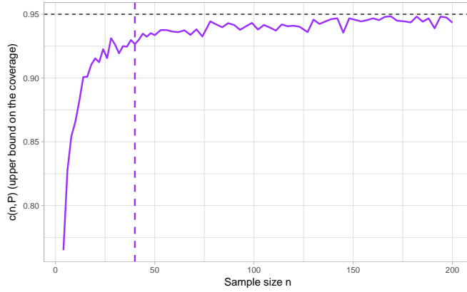
Figure 17: Specification: \forall n \in \mathbb{N}^* , the marginal distributions of X and Y are two exponentials with \mathbb{E}[X] = 1 and \mathbb{E}[Y] = 0.5 and are simulated using a Gaussian copula to have \text{Corr}(X, Y) \approx 0.75 .; 1 - \alpha = 0.95 ; 5,000 repetitions used.
