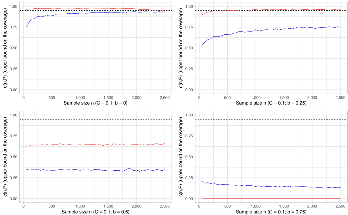
Figure 4: c(n, P) of the asymptotic CIs based on the delta method (blue) and of the CIs constructed with Efron's percentile bootstrap using 2,000 bootstrap replications (red). Specification: \forall n \in \mathbb{N}^*, P_{X,Y,n} = \mathcal{N}(1, 1) \otimes \mathcal{N}(Cn^{-b}, 1) , with C = 0.1 and b \in \{0, 0.25, 0.5, 0.75\} . The nominal pointwise asymptotic level is set to 0.95. For each pair (b, n) , the coverage is obtained as the mean over 5,000 repetitions.
