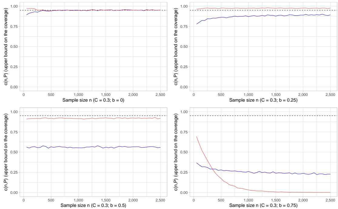
Figure 26: delta method in blue; Efron's percentile bootstrap in red; C = 0.3 .
