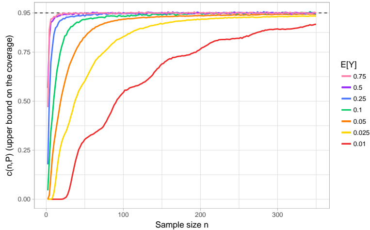
Figure 20: c(n, P) of asymptotic CIs based on the delta method as a function of the sample size n .
