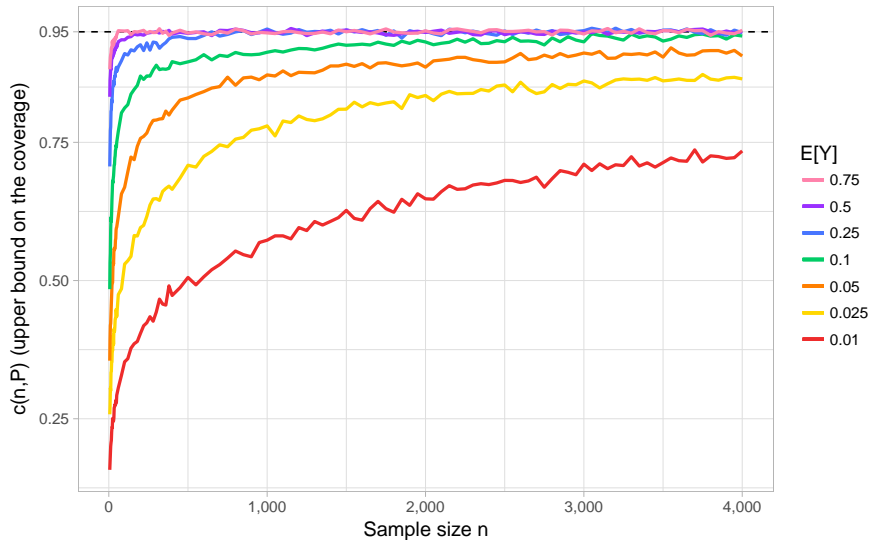
Figure 1: c(n, P) of the asymptotic CIs based on the delta method as a function of the sample size n .
