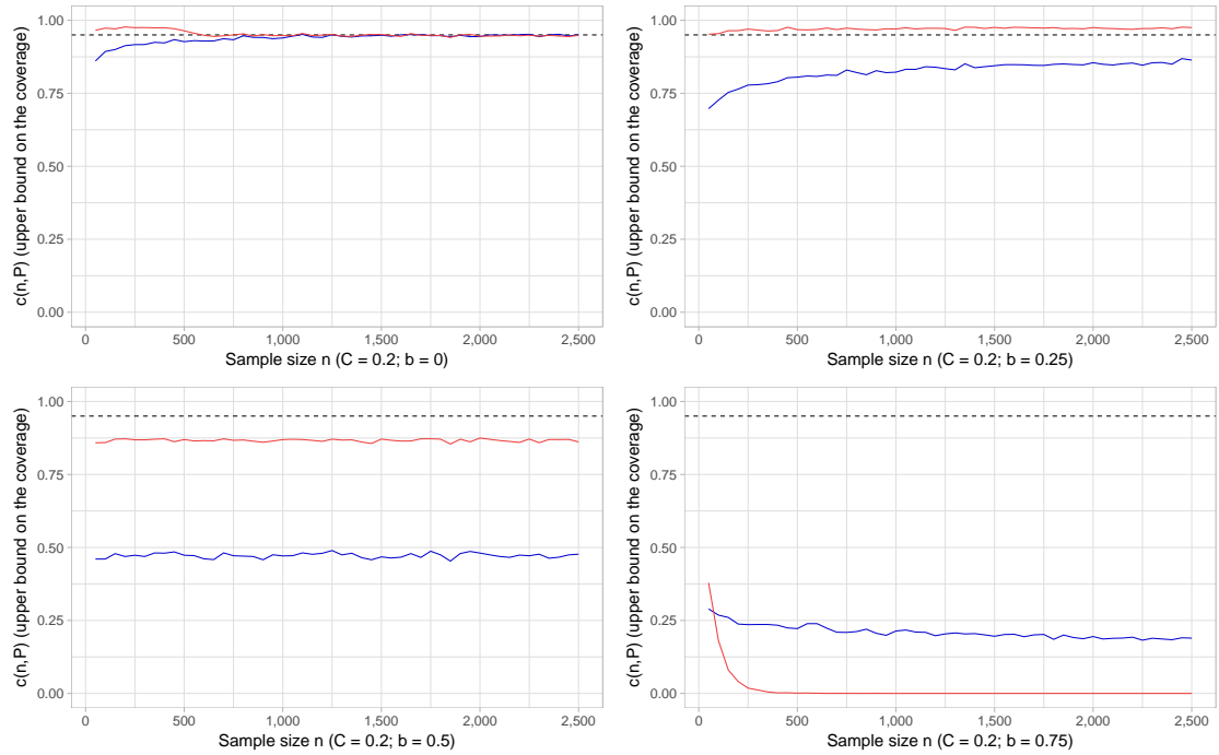
Figure 25: delta method in blue; Efron's percentile bootstrap in red; C = 0.2 .
