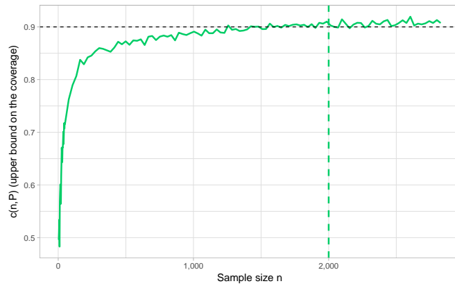
Figure 24: Specification: \forall n \in \mathbb{N}^* , the marginal distributions of X and Y are respectively \text{Poisson}(0.5, 2) and \text{Poisson}(0.1, 1) and are simulated using a Gaussian copula to have \text{Corr}(X, Y) \approx 0.6 ; 1 - \alpha = 0.9 ; 5,000 repetitions used.
