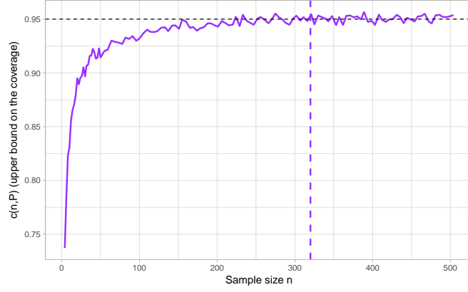
Figure 23: Specification: \forall n \in \mathbb{N}^* , P_{X,Y,n} = \text{Poisson}(0.5, 2) \otimes \text{Poisson}(0.5, 2) ; 1 - \alpha = 0.95 ; 5,000 repetitions used.
