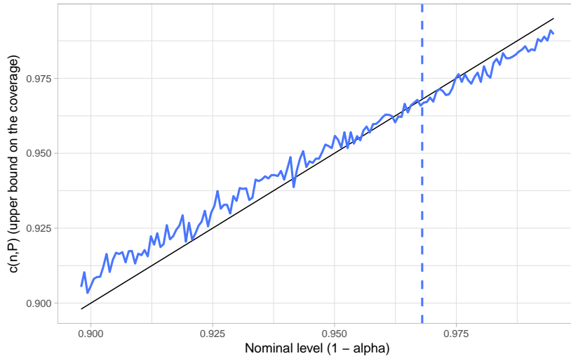
Figure 7: c(n, P) of the asymptotic CIs based on the delta method as a function of the sample size n and \bar{\alpha}_n .
