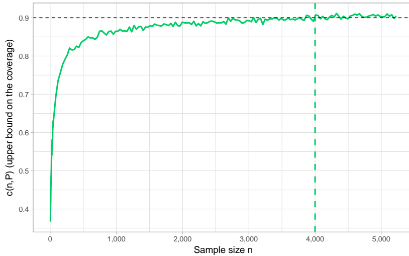
Figure 6: c(n, P) of the asymptotic CIs based on the delta method as a function of the sample size n and \bar{n}_\alpha .
