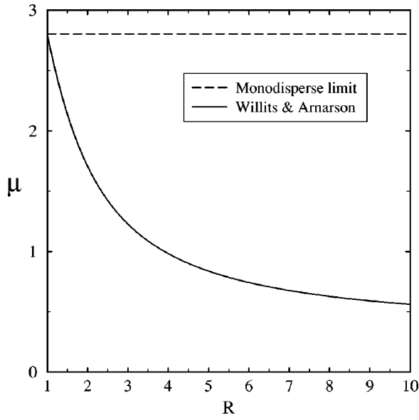
FIG. 1. Analytical results for the variation of the shear viscosity \mu with the size ratio R for uniform shear flow of an almost monodisperse mixture with volume fraction ratio \nu_l/\nu_s = 10^{14} and the total volume fraction \nu = 0.3 . The coefficient of restitution is e = 0.99 and the shear rate \gamma = 1.0 . The viscosity has been nondimensionalized by \rho_p d_l^2 \gamma , with \rho_p being the material density of the particles. The solid line corresponds to the original results of WA, and the dashed line denotes the monodisperse limit.
