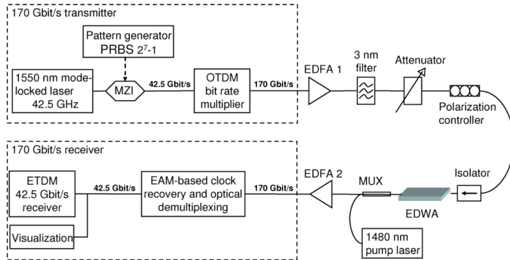
Fig. 2. Experimental setup for 170 Gbit/s transmission measurements.
