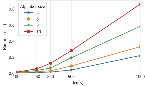
Figure 13: Runtime of the computation of \mathcal{L}_{(1,1)}(s_i, s_j) against len(s) for different values of alphabet size |\Pi| .
