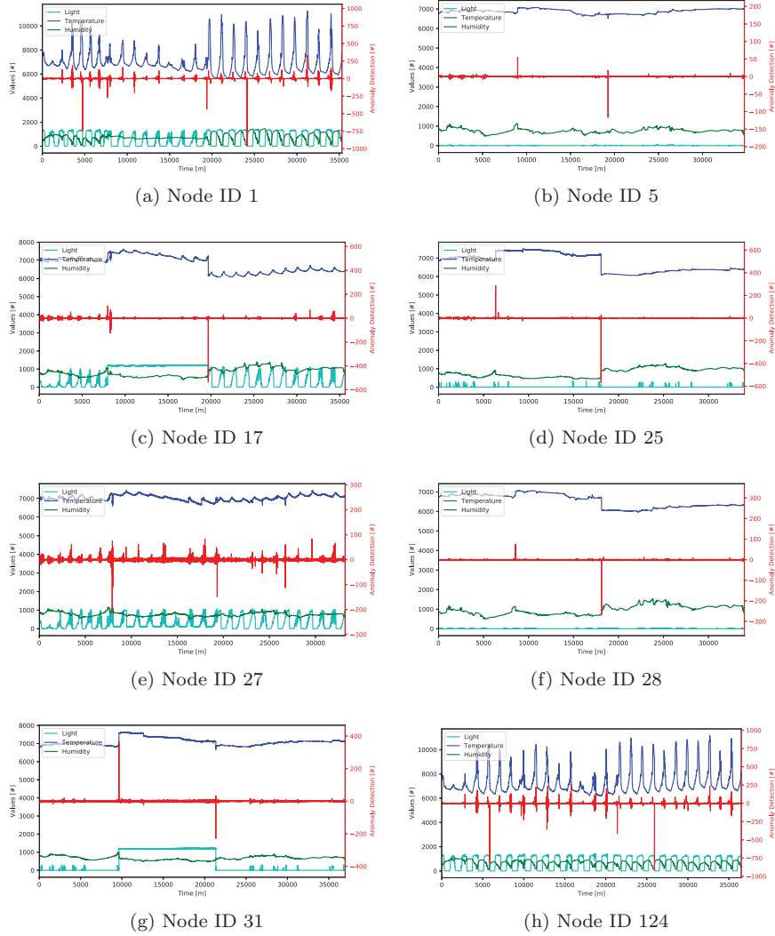
Figure 7: Short-term anomaly detection. Each subplot reflects how our proposed method, Anomaly detection with Generative Replay (AnGe), detects anomalies on a specific node. The x-axes represent the time, the left y-axes show the sensors measurements, while the right y-axes (red) show the values of m_{AnGe} .
