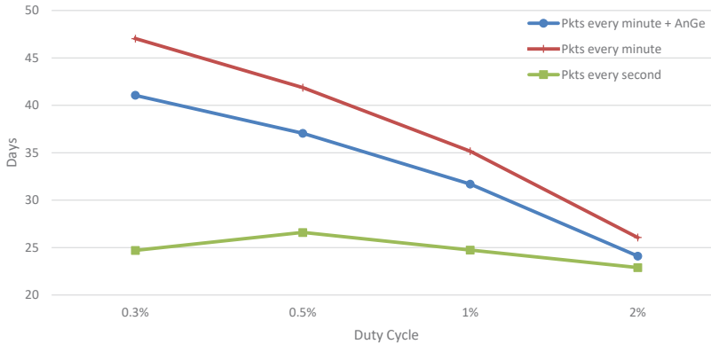
Figure 8: Comparison of battery lifetimes, considering different duty cycles, for TelosBs running the BMF and (i) sending pkts per second, (ii) sending pkts per minute, and (iii) sending pkts per minute + elaborating the AnGe Function.
