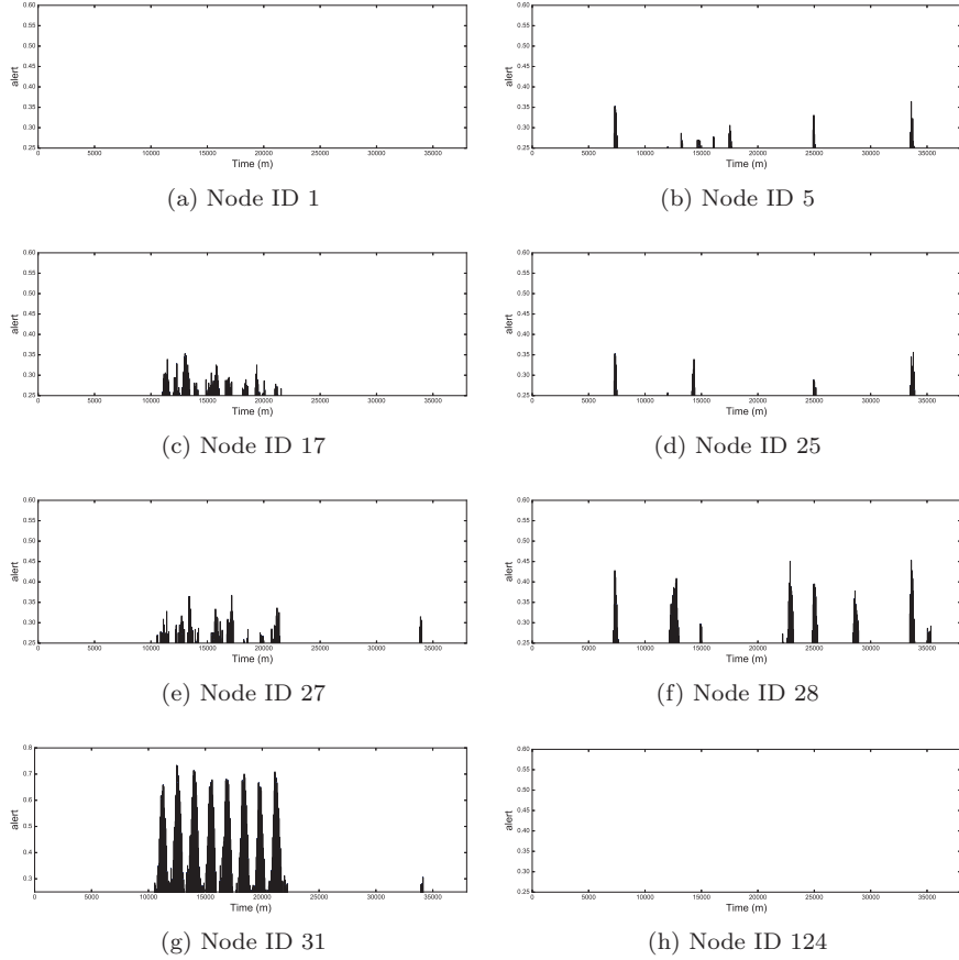
Figure 9: Alerts (with over-threshold values) for long-term anomaly detection of light sensors. The x-axis represents the time, the y-axis indicates the value of |\chi(s_i, h', d) - \eta(s_i, h')| .
