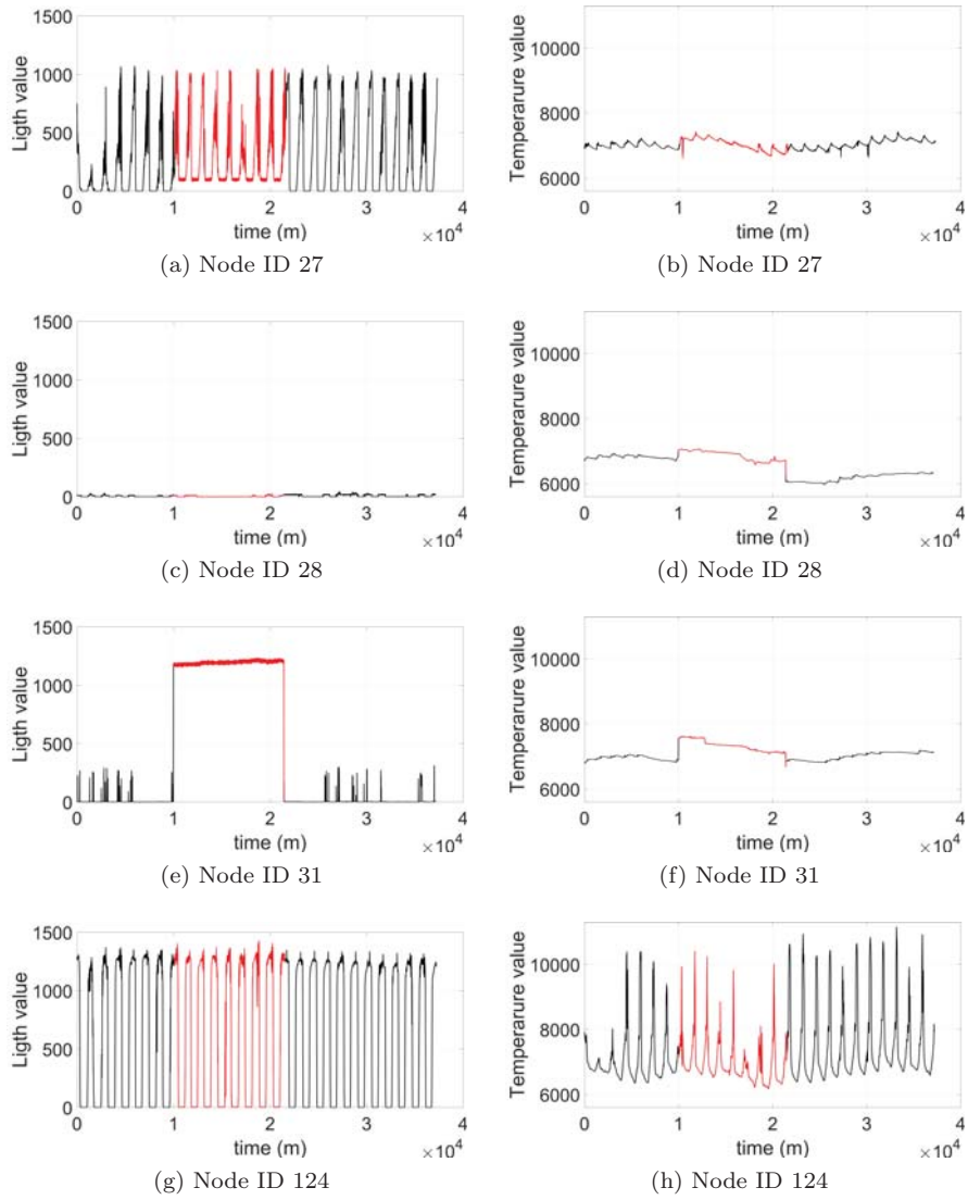
Figure 5: Light and temperature raw sensor data for node identifiers 27, 28, 31, and 124. The temporal window corresponding to the application of interferences to sensors 1, 5, 17, and 31 is highlighted in red for all the plots.
