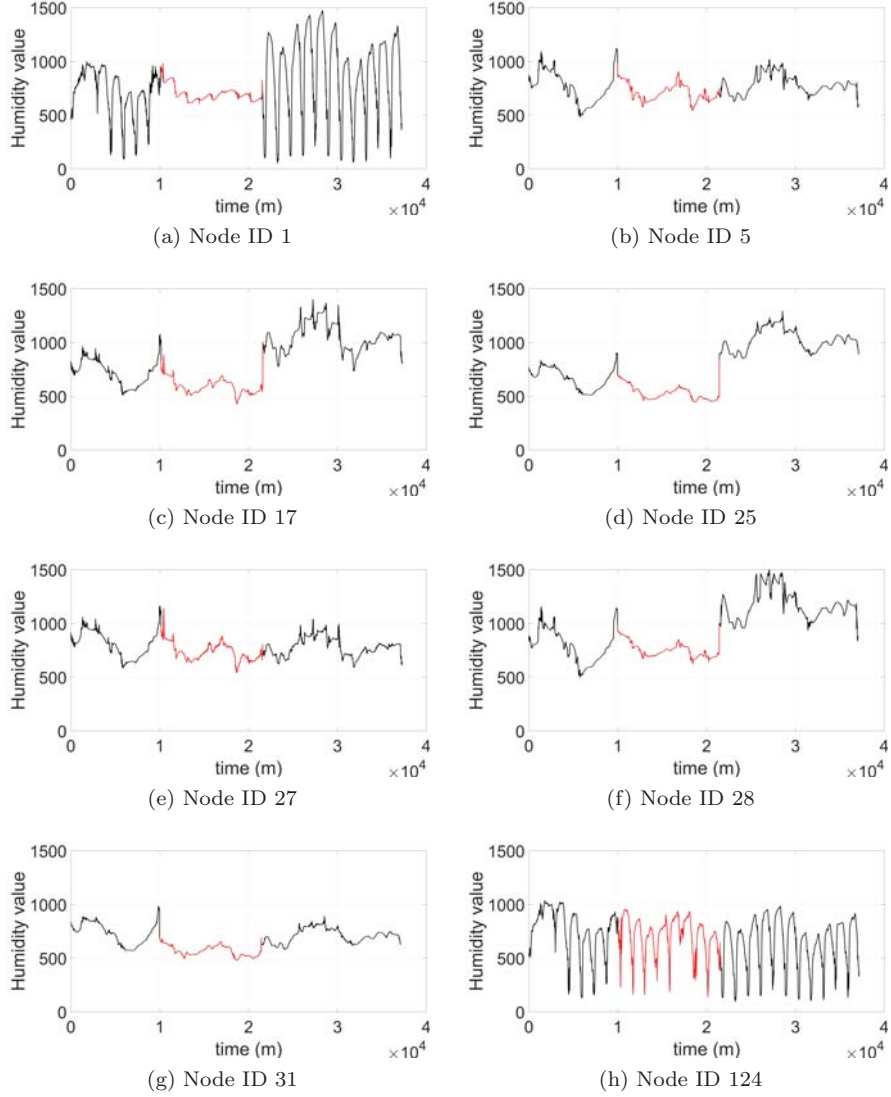
Figure 6: Humidity raw sensor data for node identifiers 1, 5, 17, 25, 27, 28, 31, and 124. The temporal window corresponding to the application of interferences to sensors 1, 5, 17, and 31 is highlighted in red for all the plots.
