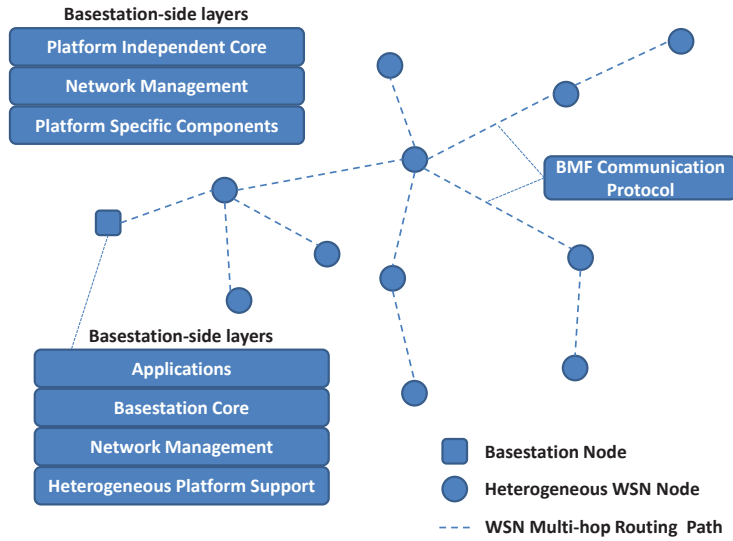
Figure 2: A BMF Network example.
