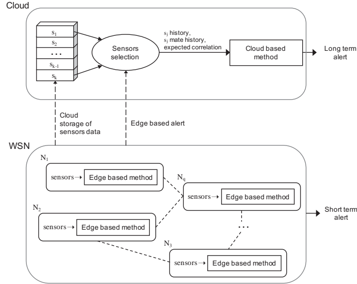
Figure 1: The main workflow of the proposed approach.
