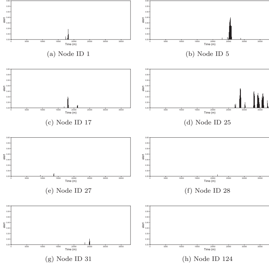
Figure 10: Alerts (with over-threshold values) for long-term anomaly detection of temperature sensors. The x-axis represents the time, the y-axis indicates the value of |\chi(s_i, h', d) - \eta(s_i, h')| .
