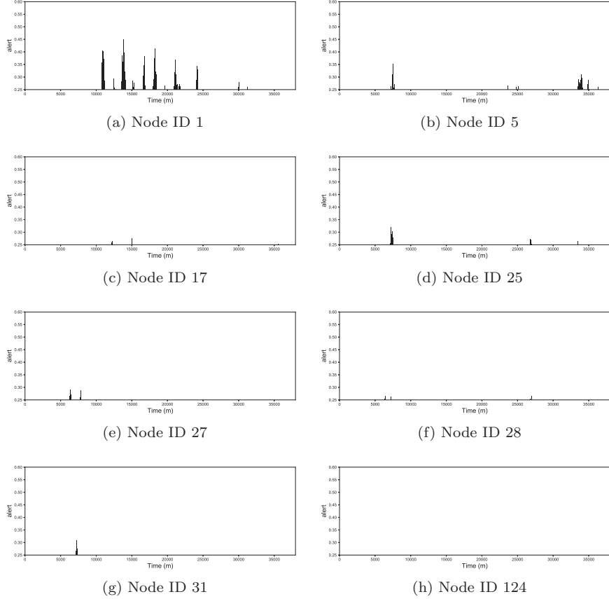
Figure 11: Alerts (with over-threshold values) for long-term anomaly detection of humidity sensors. The x-axis represents the time, the y-axis indicates the value of |\chi(s_i, h', d) - \eta(s_i, h')| .
