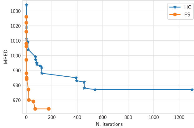
Figure 12: Comparison of two heuristics for MPED, ES and HC, with |\Pi| = 14 len(s) = 2000 and \pi_1 = \pi_2 = 4 .
