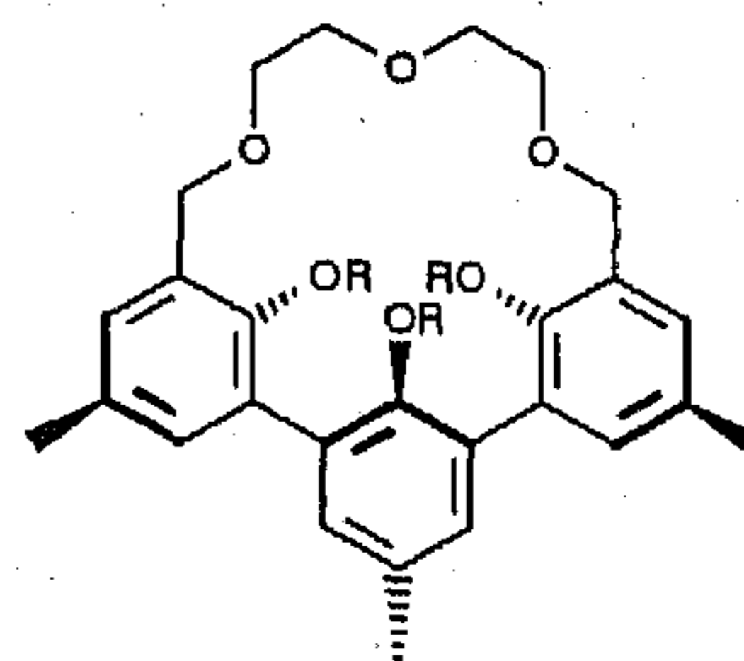
1 R = \text{CH}_2\text{COOEt} 2 R = Me
