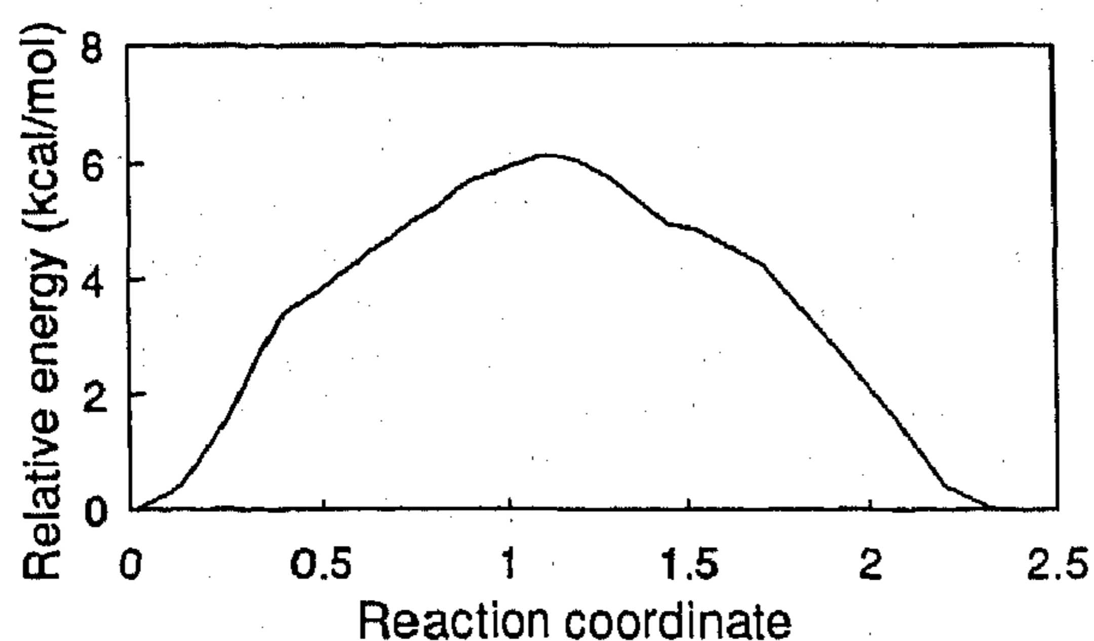
Fig. 5 Energy profile of fast exchange process
