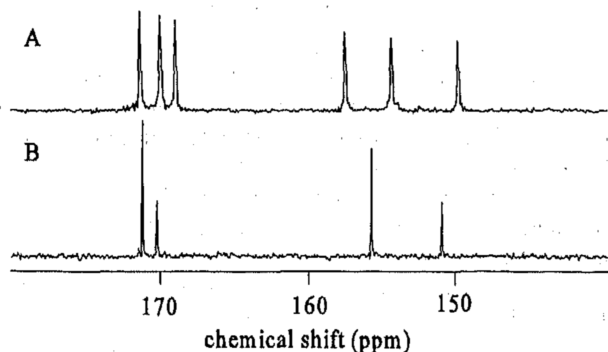
Fig. 2 ^{13}\text{C} NMR spectra of 1 \cdot \text{NaClO}_4 ; (a) solid state (CPMAS) and (b) in \text{CD}_3\text{OD} solution
