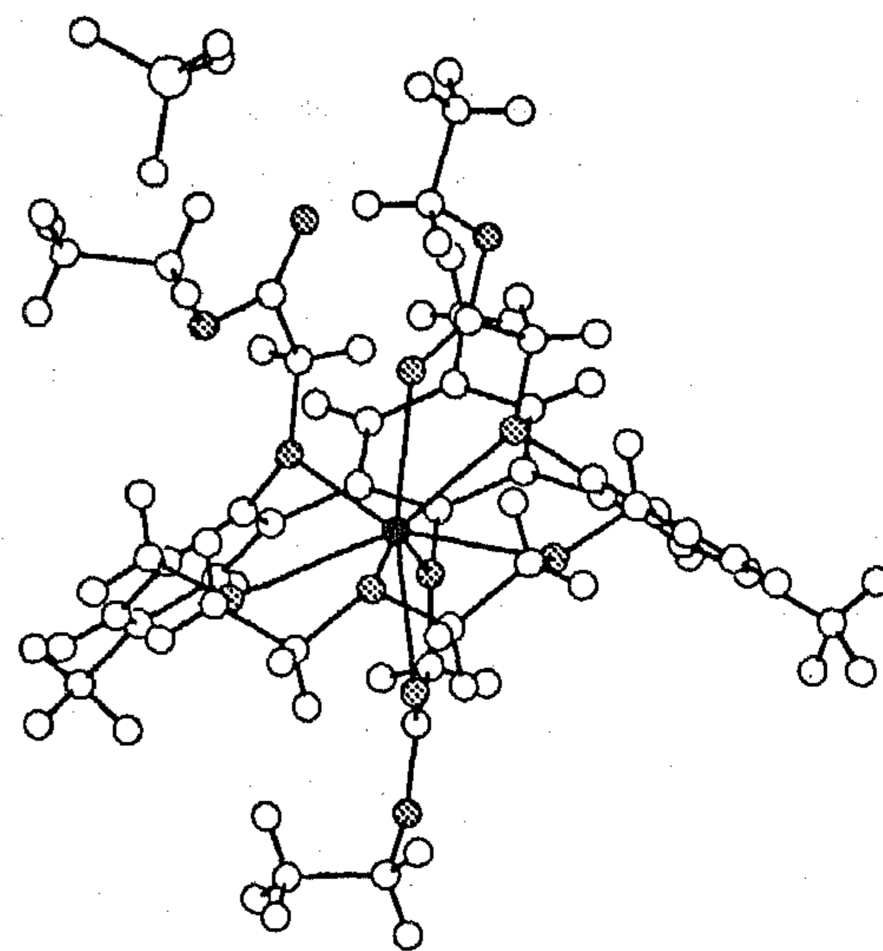
Fig. 1 X-Ray structure of 1·NaClO 4
