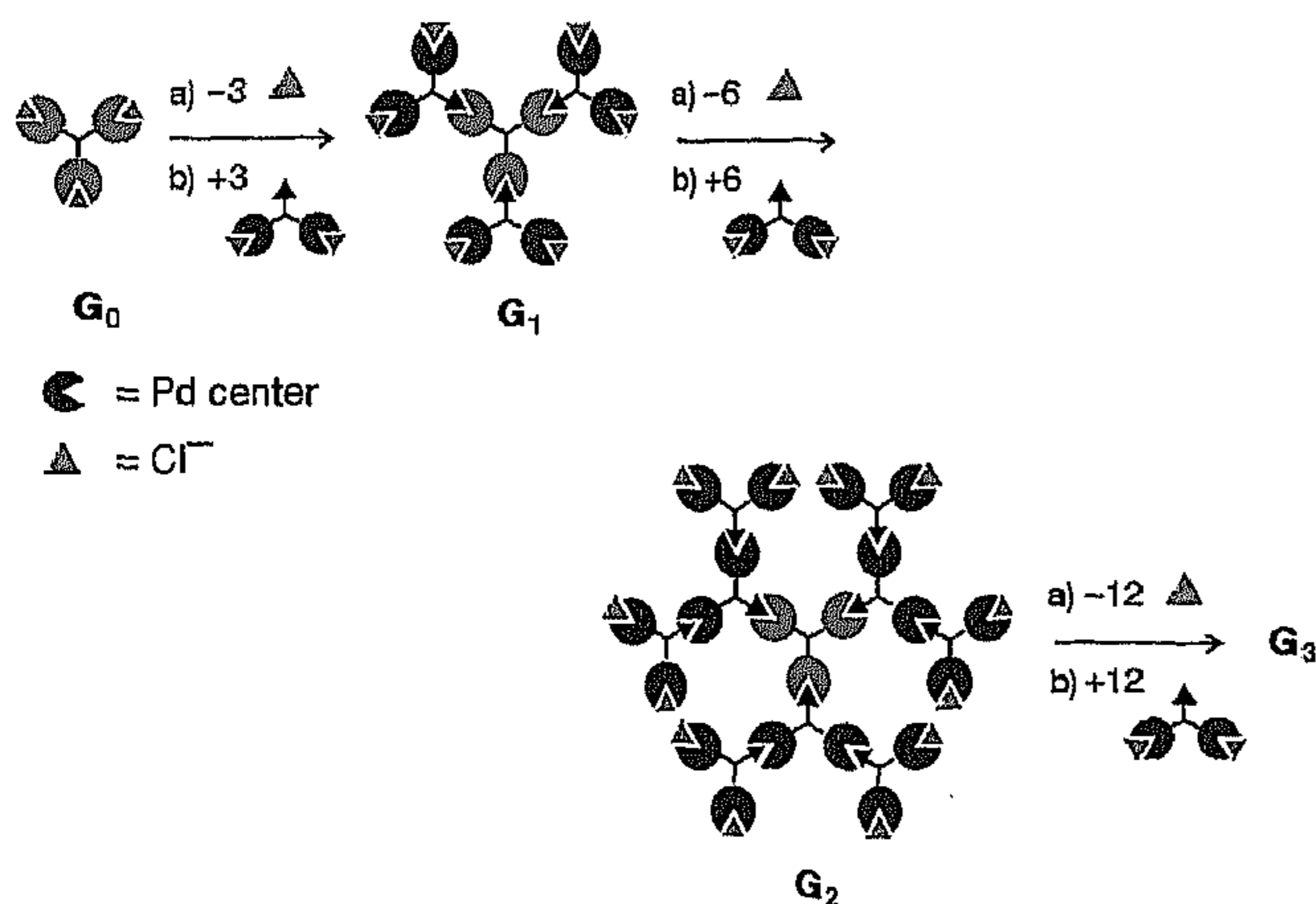
Scheme 2. Synthesis of dendrimer building blocks.
