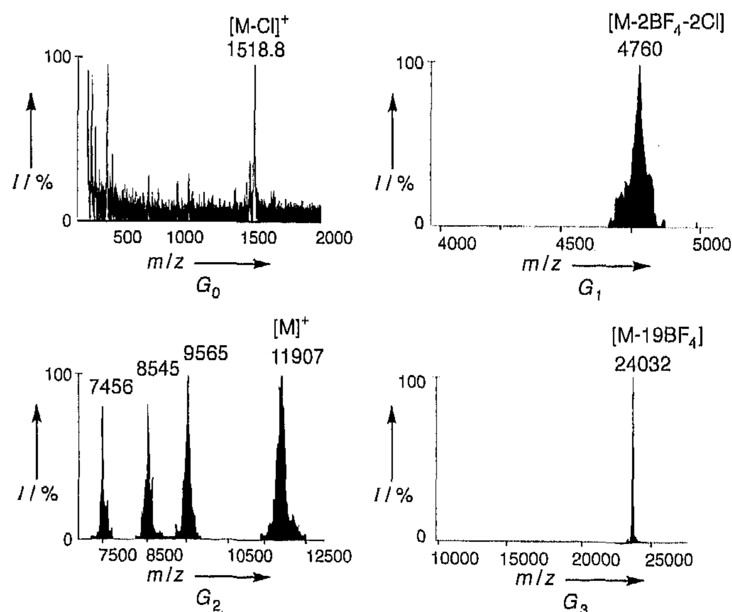
Fig. 1. ES mass spectra for G_1 – G_3 .
