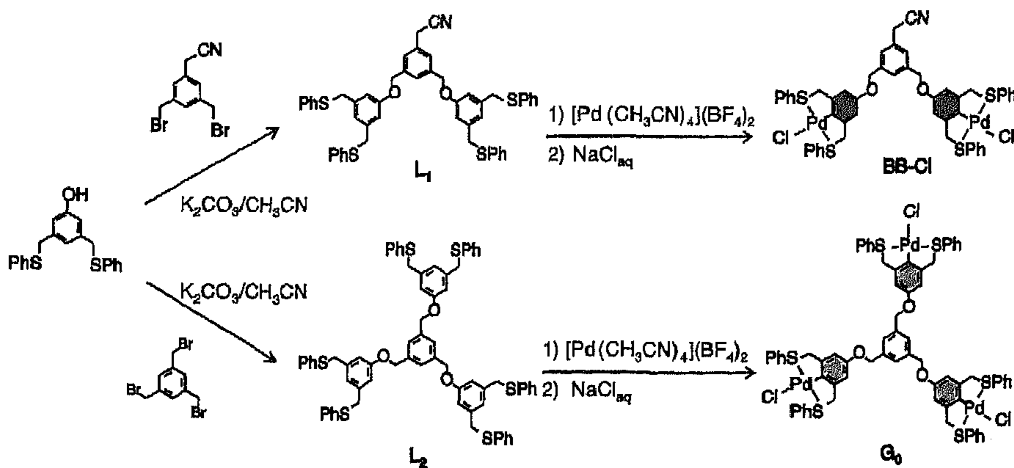
Scheme 1. Graphical representation of the controlled assembly process.
