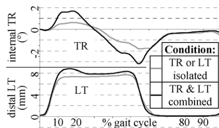
Fig. 1. Pattern of TR and LT at the adapter (displacement of the socket relative to the foot).
