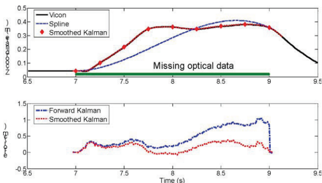
Fig. 1. Two seconds of gap filling with a spline function and inertial data (upper) and the Kalman errors (lower).
