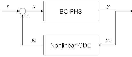
Fig. 1. Power preserving interconnection.
