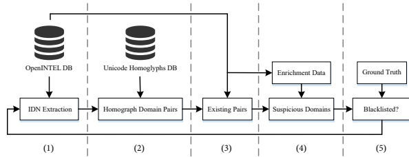
Figure 1. High-level overview of the proposed method
