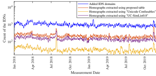
Figure 3. Extracted homographs for added IDNs
