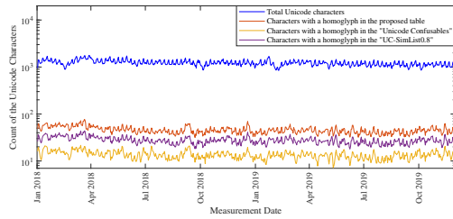
Figure 4. Characters with a homograph for added IDNs
