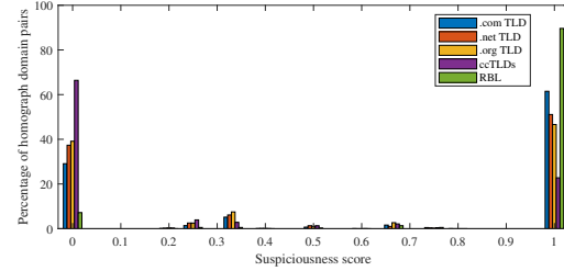
Figure 5. Suspiciousness score for extracted and blacklisted domains
