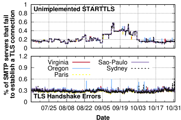
Figure 6: The percentage of the established SMTP connections that fail to initiate TLS connections is shown.
