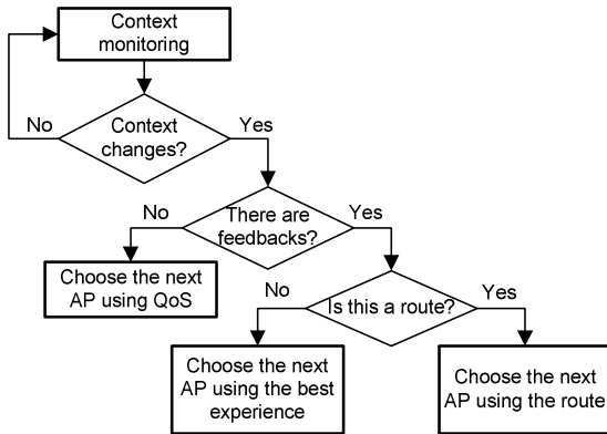
Figure 2. Flowchart summarizing the actions on move
