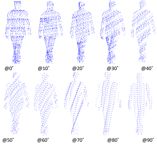
Fig.9. Point clouds of a standing person at different orientation angles of the LiDAR 10 meters aside from the mobile mapping vehicle trajectory.
