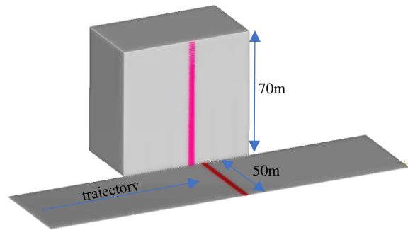
Fig.4. The simulated road and building façade and two selected slices for testing the point density.
