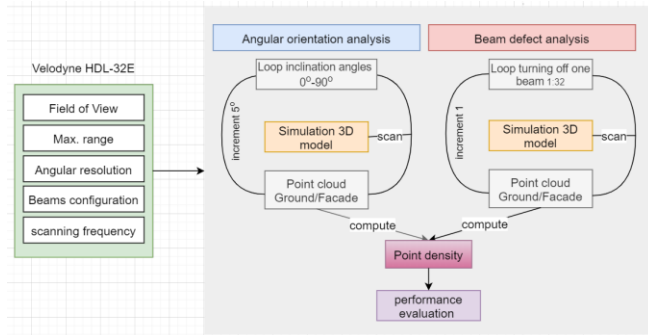
Fig. 5. Methodology workflow.
