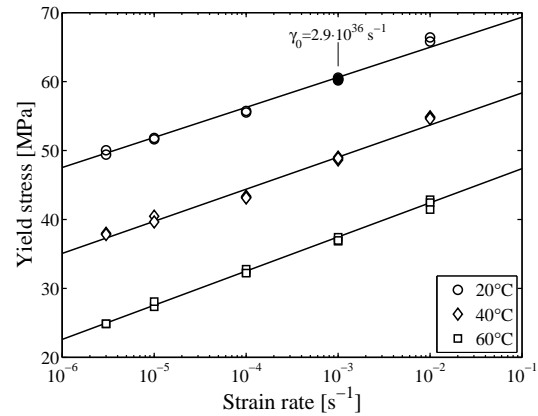
Figure 4: Tensile yield stress of uPVC for various strain rates at three temperatures. The solid lines represent the best fit using (1)
