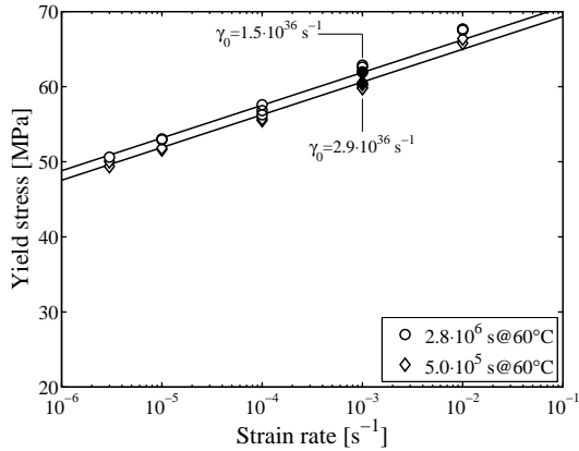
Figure 6: Engineering yield stress versus strain rate measured at a temperature of 20°C for uPVC samples with different thermal histories.
