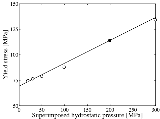
Figure 3: The yield stress of uPVC as measured in tension with a superimposed hydrostatic pressure as measured by Yuan et al. [24]. The solid line is a fit using (4) and \mu = 0.14 .
