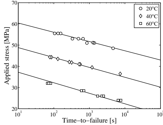
Figure 5: Results of tensile static fatigue experiments on uPVC at three temperatures. The solid lines represent the best fit of the model using the critical strain as the fit parameter
