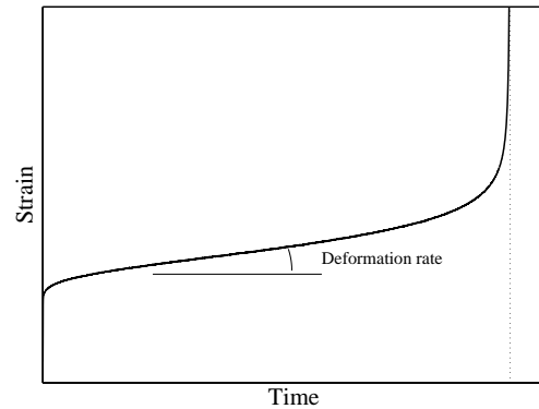
Figure 2: Typical result of static fatigue tests as carried out in tension. The anelastic deformation rate is shown in the figure. The dotted line indicates where failure occurs.
