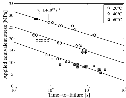
Figure 8: Time-to-failure data originating from pressurised pipes tests on uPVC, as measured by Niklas et al. [5]. The unfilled, grey and black markers represent ductile, semi ductile and brittle failure respectively. The solid lines are predictions using equation 6.
