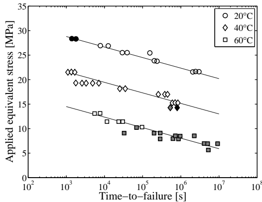
Figure 1: Time-to-failure data originating from pressurised pipes tests on uPVC, as measured by Niklas et al. [5]. The unfilled, grey and black markers represent ductile, semi ductile and brittle failure respectively. The lines serve as guides to the eye.
