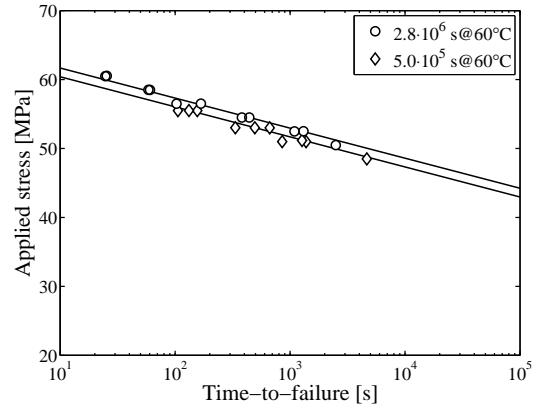
Figure 7: Time-to-failure versus the applied stress as measured with tensile static fatigue test at 20°C for uPVC samples with different thermal histories
